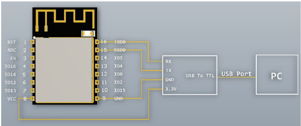
Figure 7 ESP-12S connect with computer
