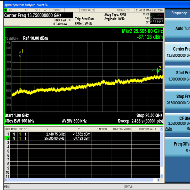
2DH5-Ant1-2441-1000~26500-PASS
