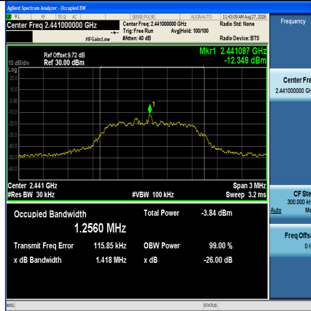
2DH5-Ant1-2441
