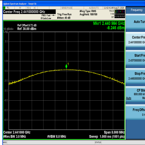
2DH5-Ant1-2441-PASS
