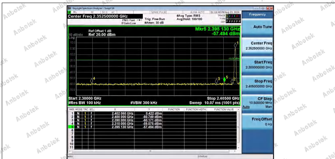
DH5-Ant1-2402-PASS
