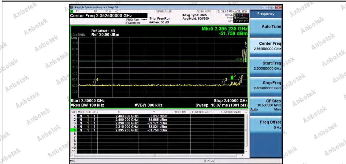
DH5-Ant1-Hop_2402-PASS
