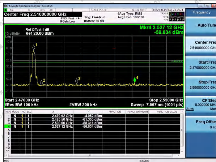
3DH5-Ant1-2480-PASS
