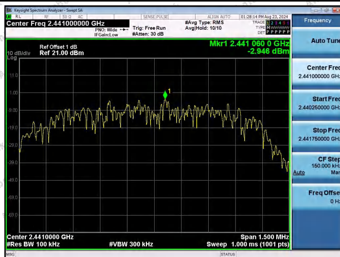
3DH5-Ant1-2441-0~Reference-PASS
