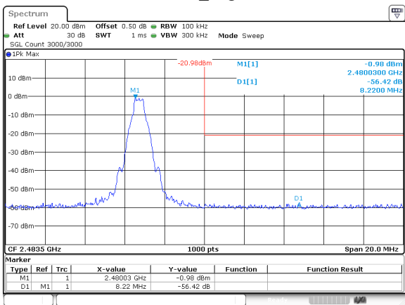
DH1_High
