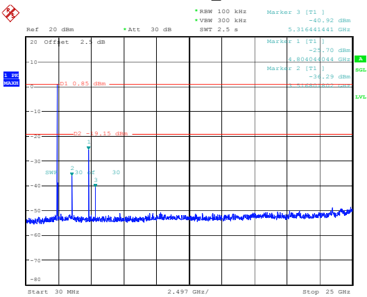
2DH1_Low
