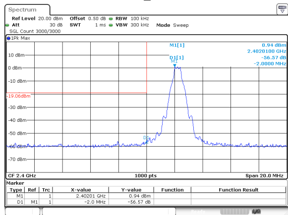
DH1_Low
