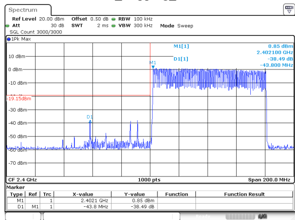
DH1_Hopping_Lower
