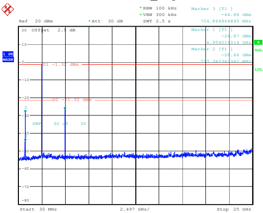
2DH1_High
