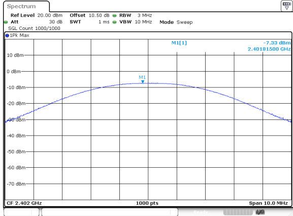
BLE_1M_Low_Channel
