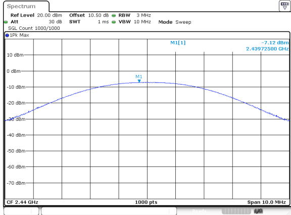
BLE_1M_Middle_Channel
