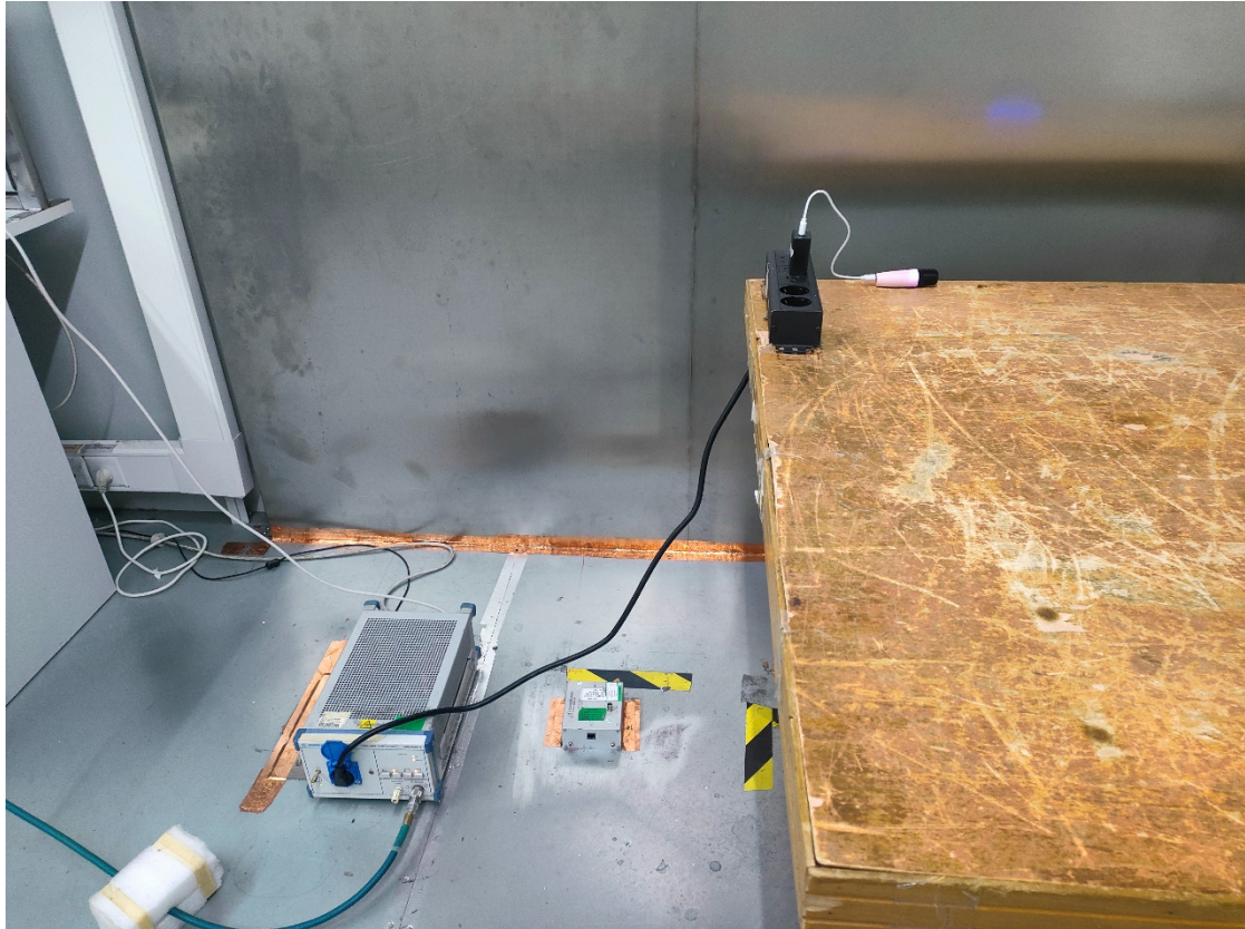
AC Line Conducted Emissions - Side View
