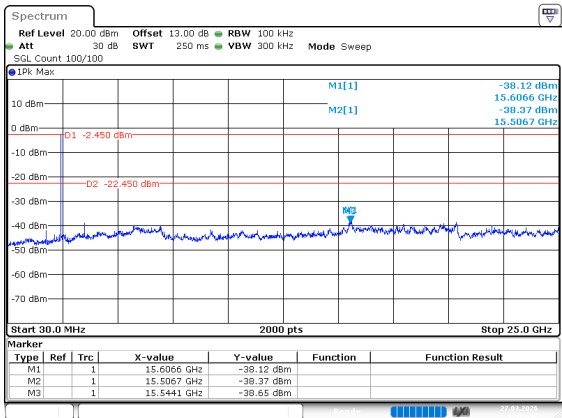
BLE_1M_Middle_Channel
