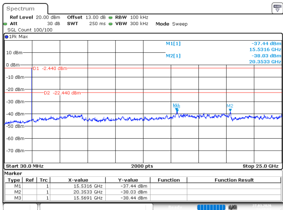
BLE_1M_High_Channel
