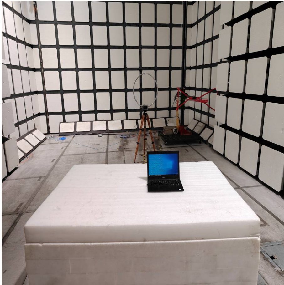
Radiated Emissions View (30 MHz- 1 GHz)
