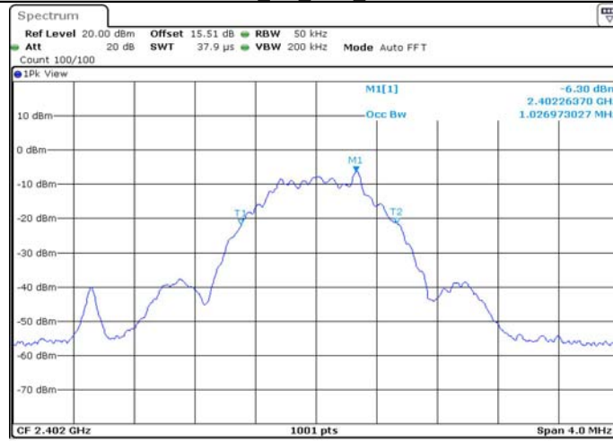
BLE_1M_Ant1_2402
