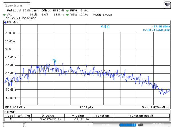
BLE_1M_Low_Channel
