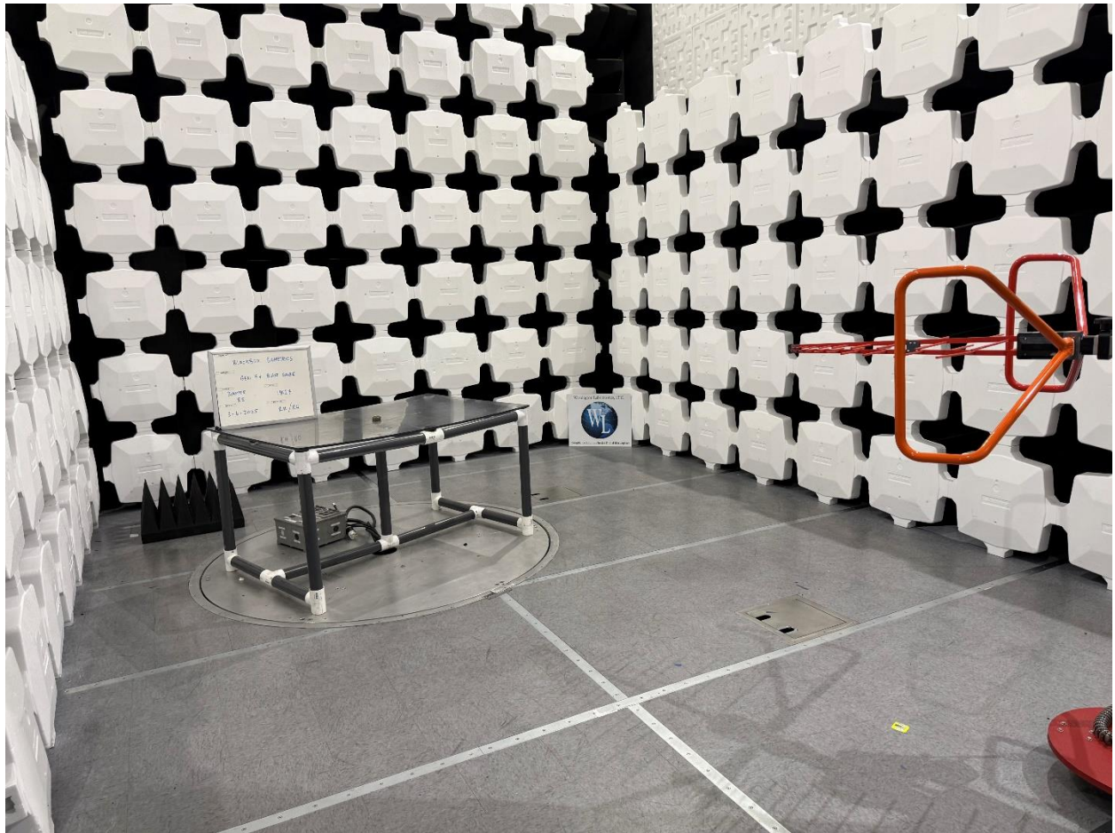
Radiated Testing, 30MHz to 1GHz, View 1
