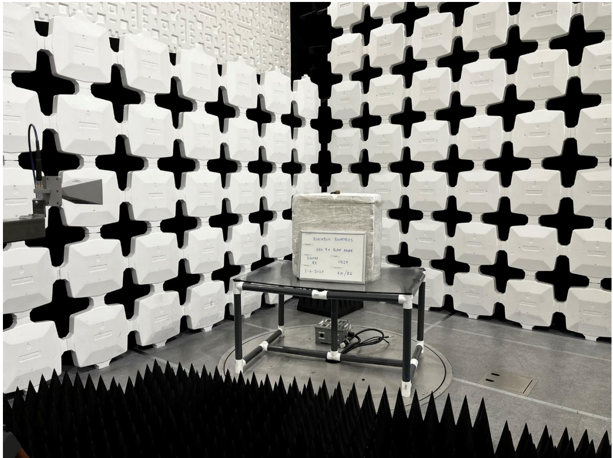
Radiated Testing, 12GHz to 26.5GHz, View 1
