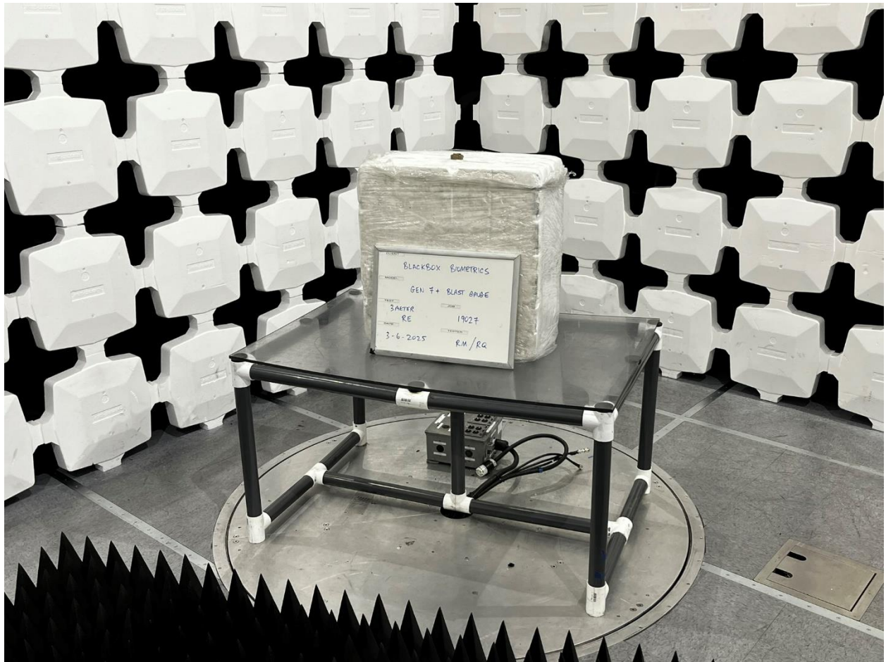
Radiated Testing, 12GHz to 26.5GHz, View 2
