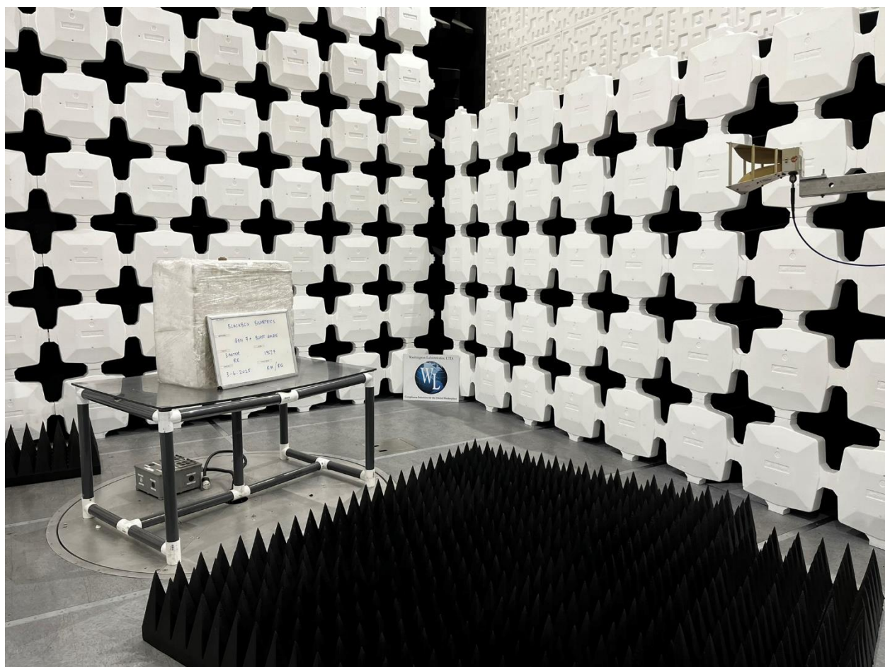
Radiated Testing, 1GHz to 12GHz, View 1
