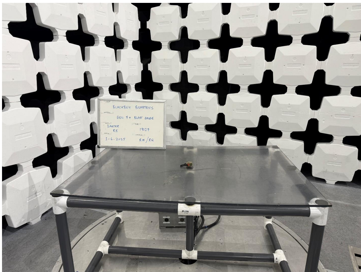
Radiated Testing, 30MHz to 1GHz, View 2
