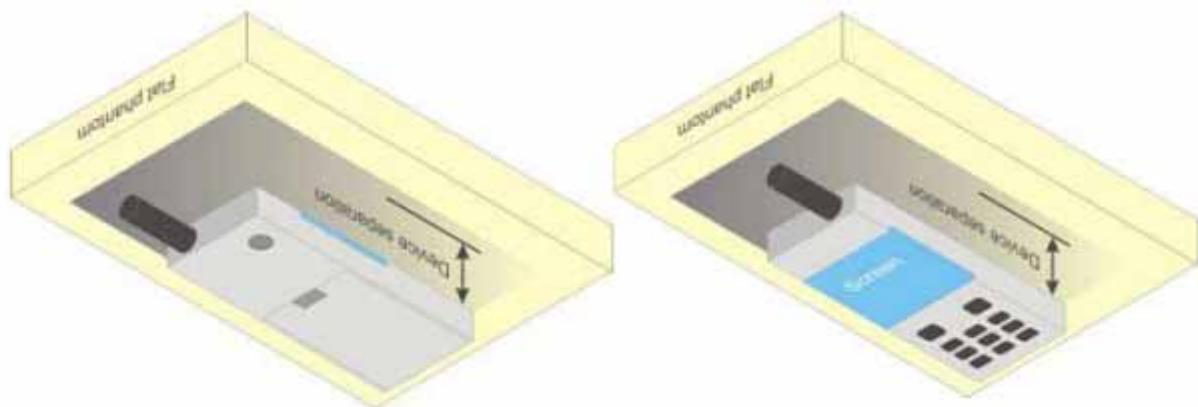
Figure 6.1 – Test positions for Wrist-Worn devices
