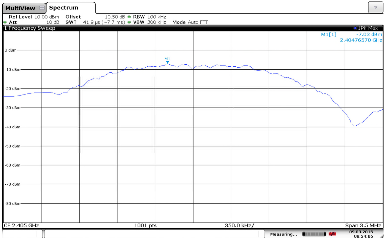
PSD Measurement - 2405MHz
