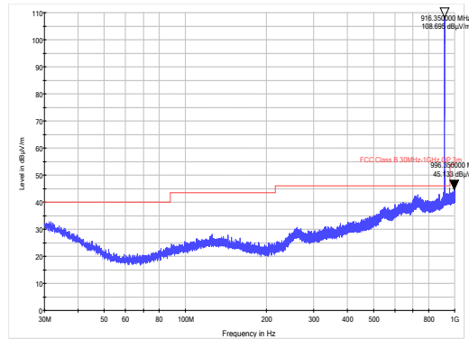
1 – 916.5 MHz (30 MHz to 1 GHz).
