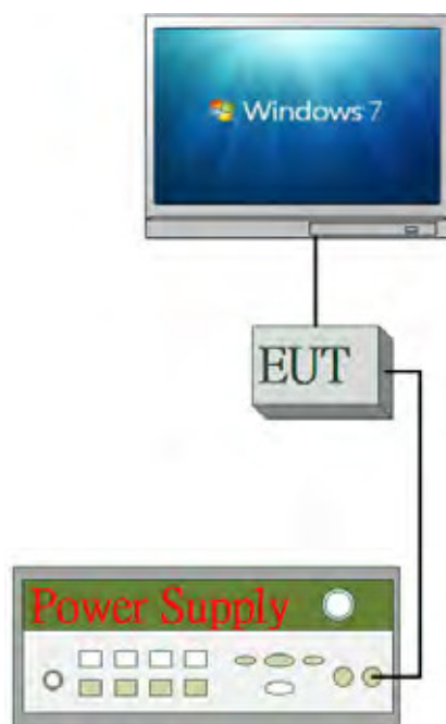
Fig. 2-2 Conducted Emission
