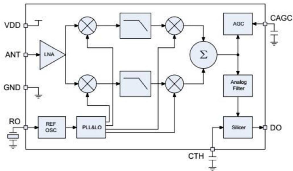
433.87MHz receiver block diagram
