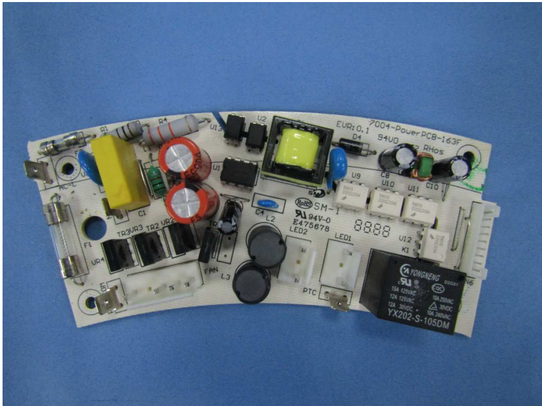
Power circuit PCBA view
