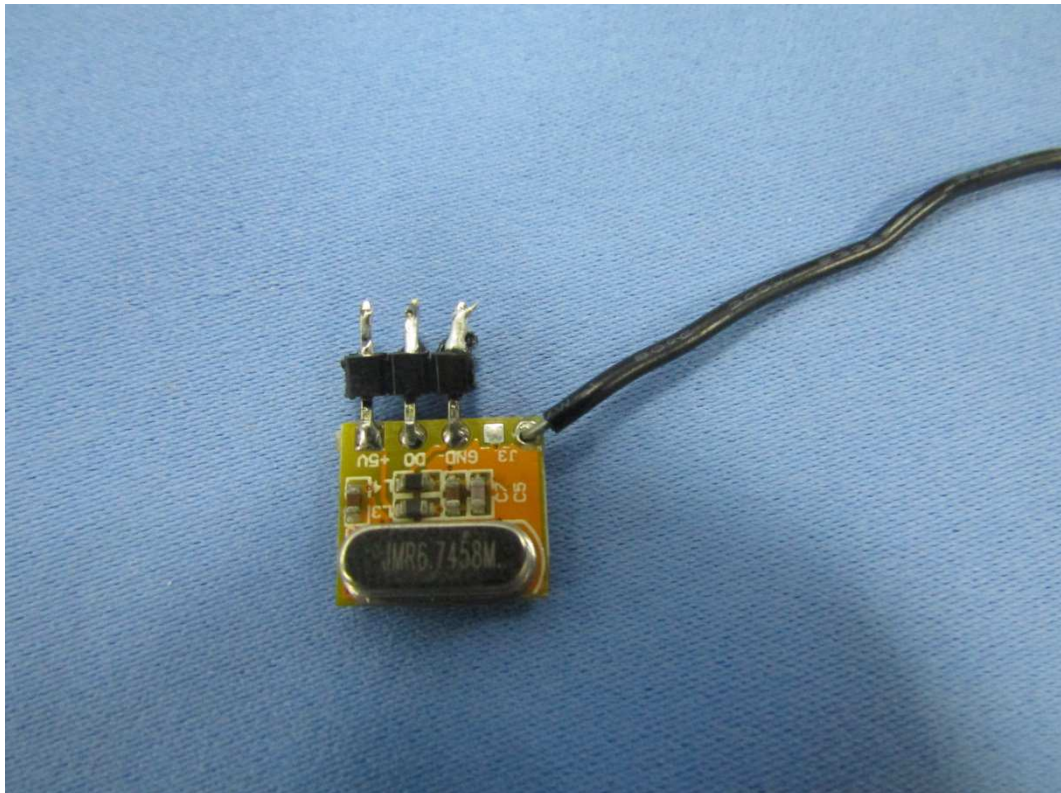
433MHz receiver module PCBA view
