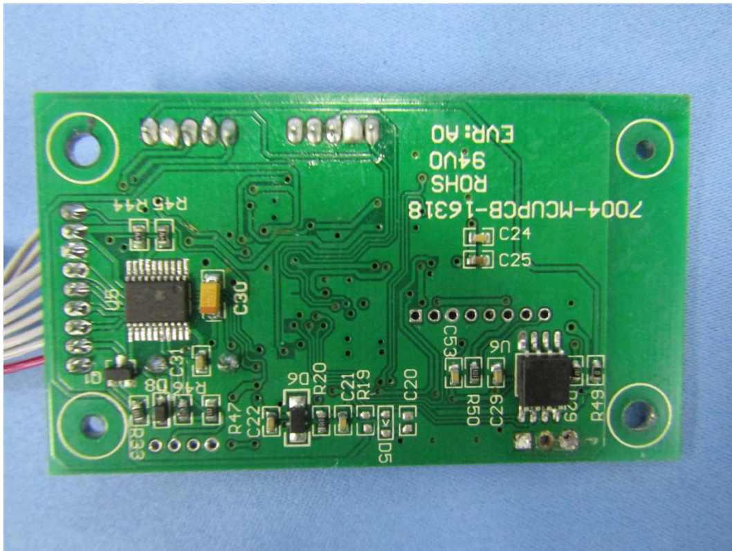
Control circuit PCBA view
