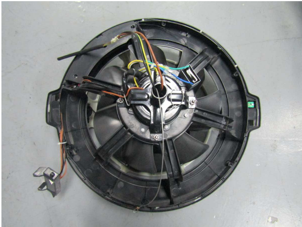
Inside view
