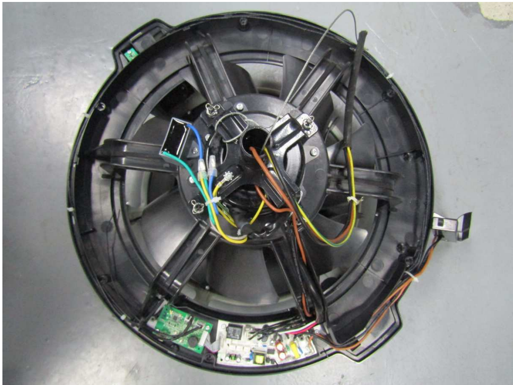
Circuit view
