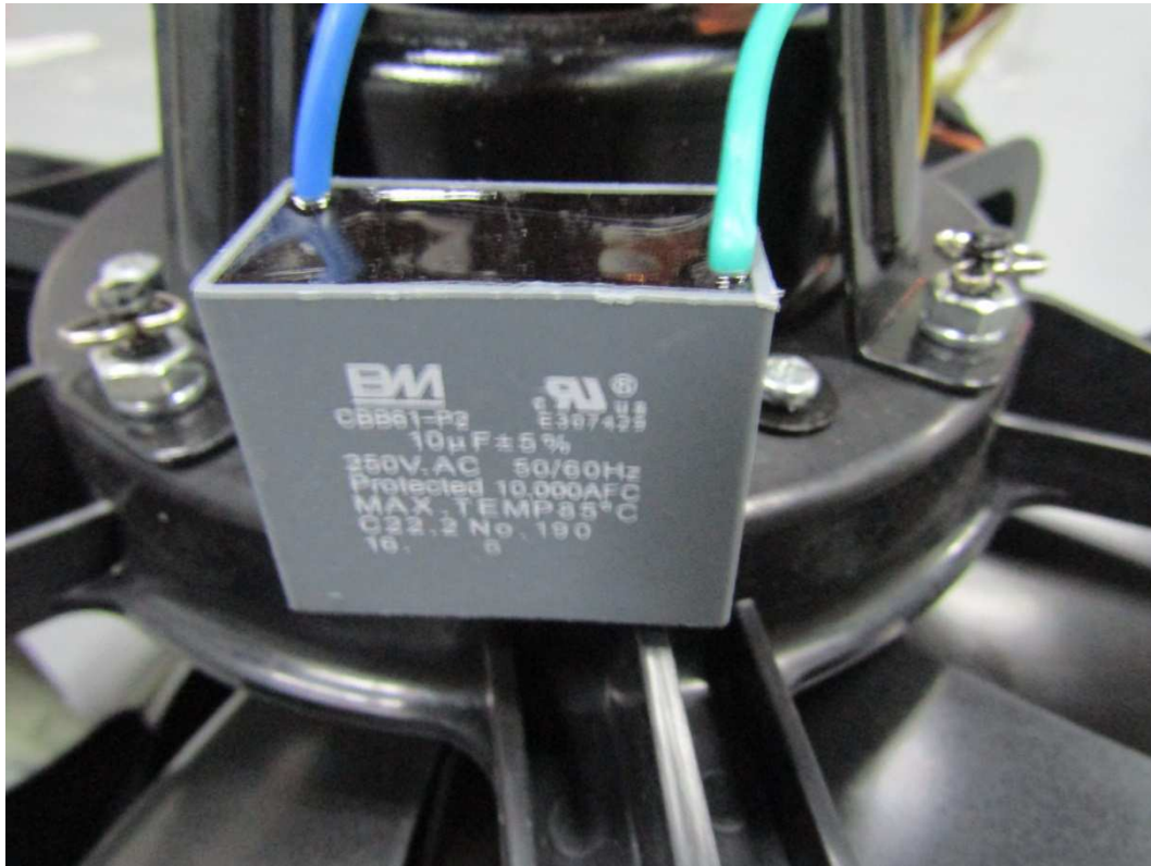
Motor capacitance view
