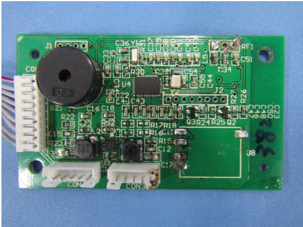
Control circuit PCBA view (removed the WIFI module and 433MHz receiver module)
