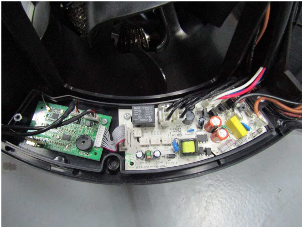
Circuit view
