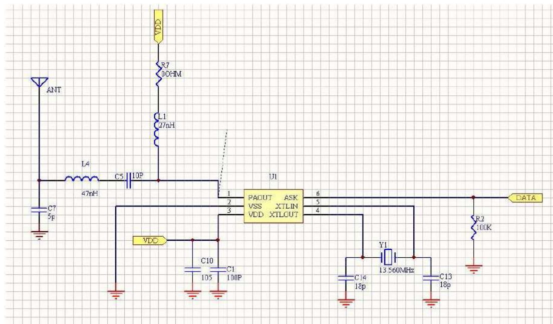
U2 TX60 circuit
