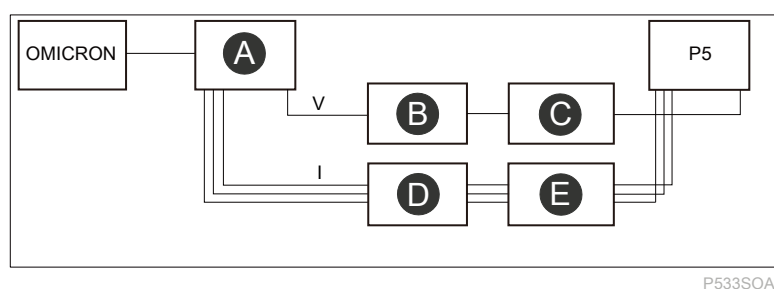
Figure 154 - LPCT/LPVT testing with test sockets/plugs
