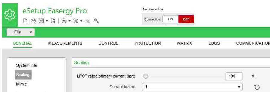
Figure 132 - LPCT setting
