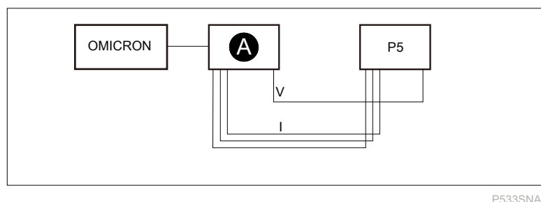
Figure 153 - LPCT/LPVT direct testing without test sockets/plugs
