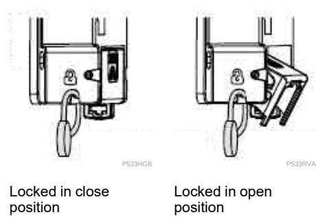
Figure 115 - RJ45 terminal lock
