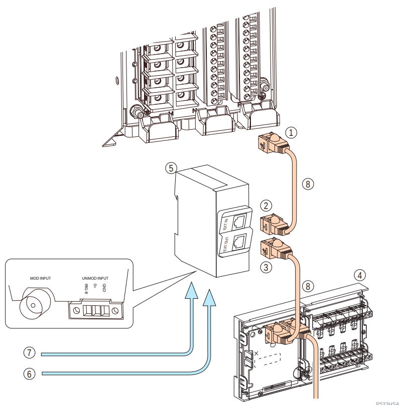
Figure 127 - Connection of IRIG-B
