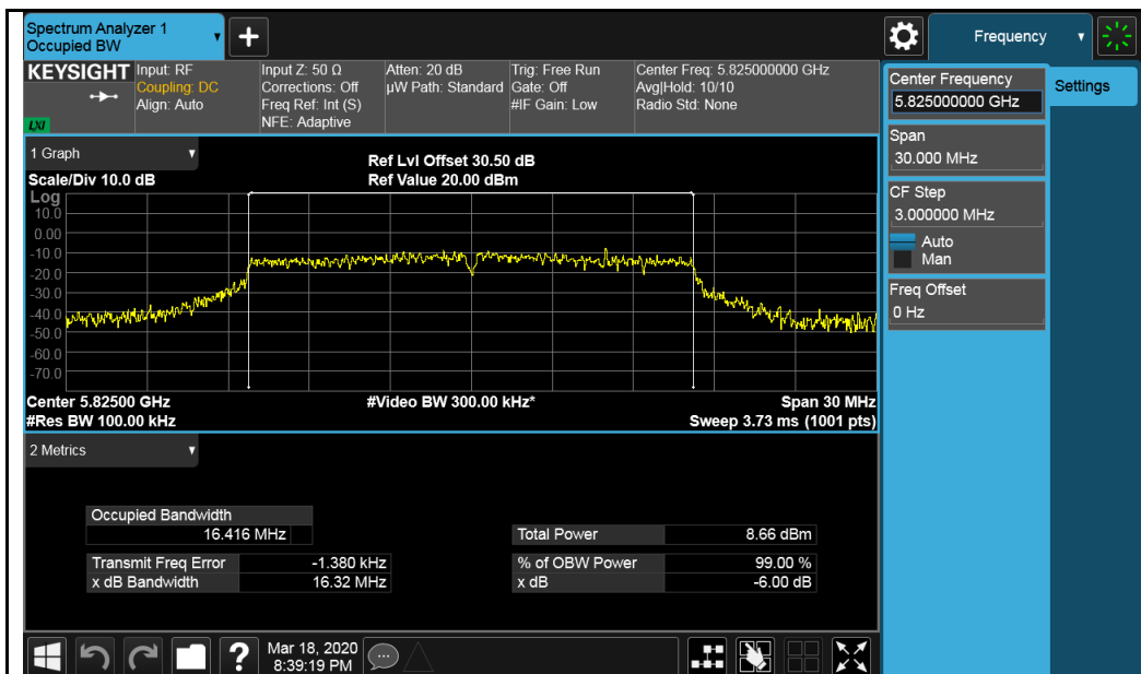
802.11a-5825MHz
