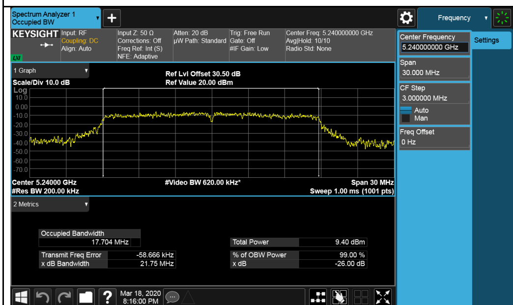
802.11n-HT20-5240MHz
