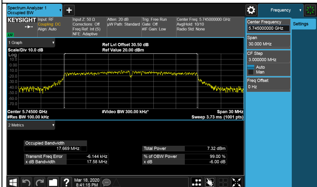
802.11n-HT20-5745MHz
