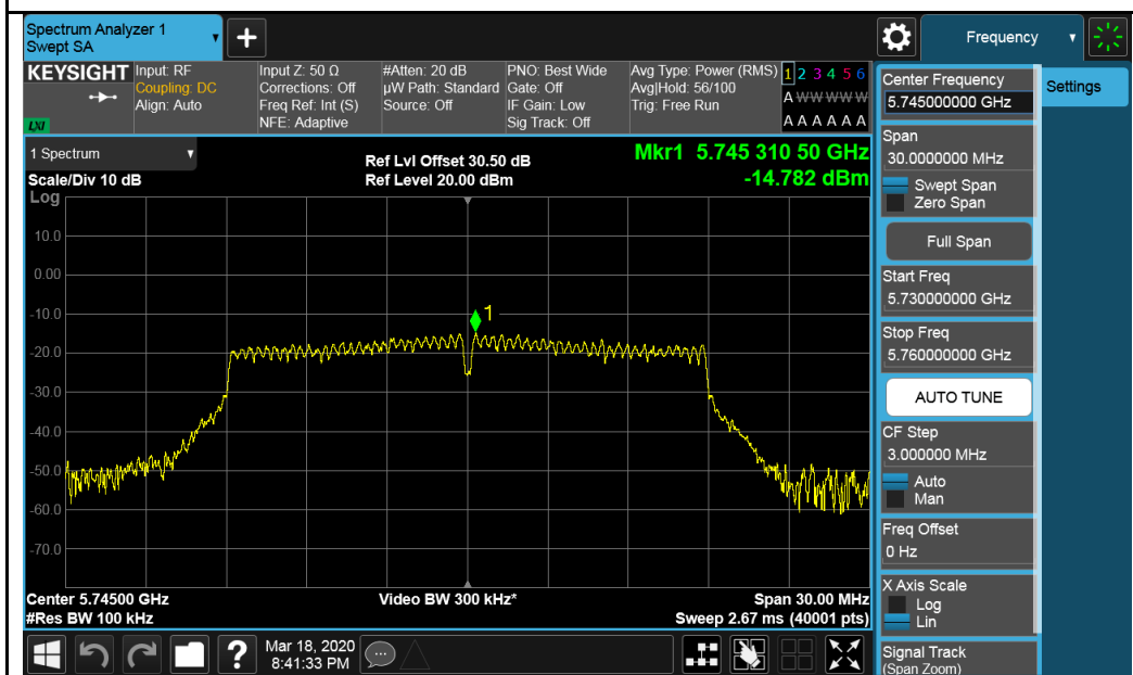
802.11n-HT20-5745MHz
