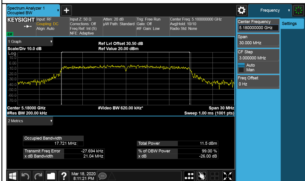
802.11n-HT20-5180MHz
