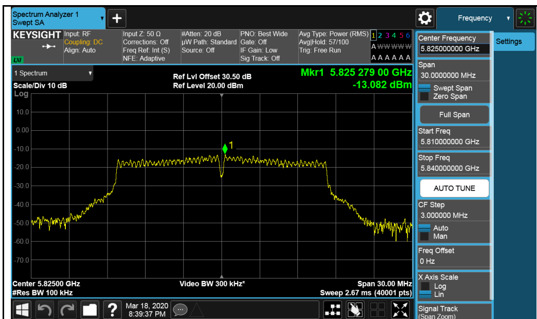
802.11a-5825MHz
