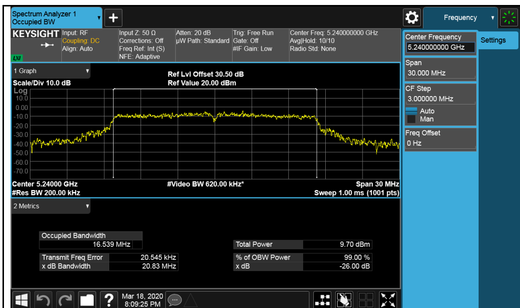
802.11a-5240MHz
