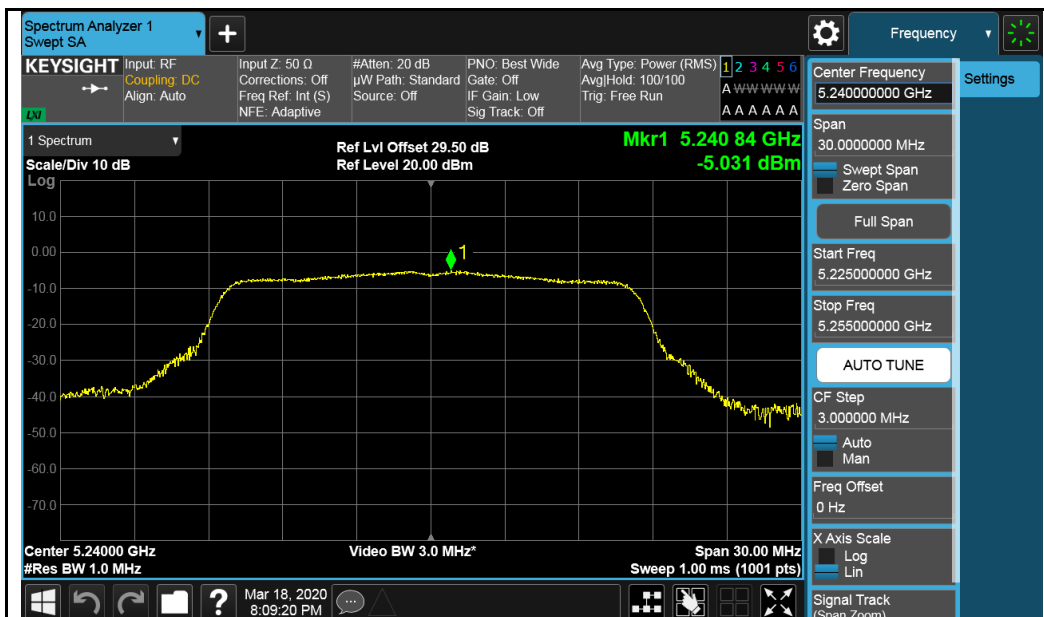
802.11a-5240MHz
