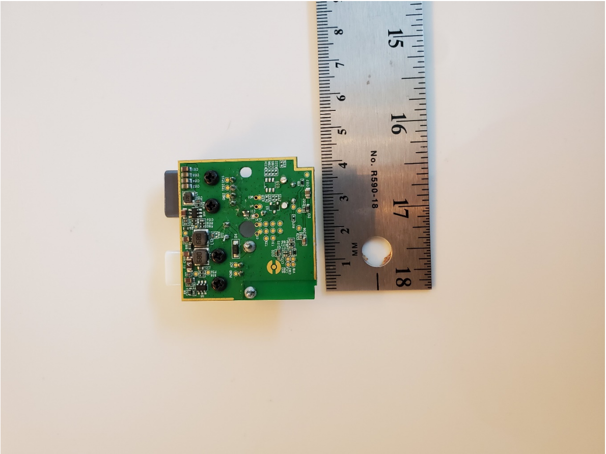
PCB Side 2
