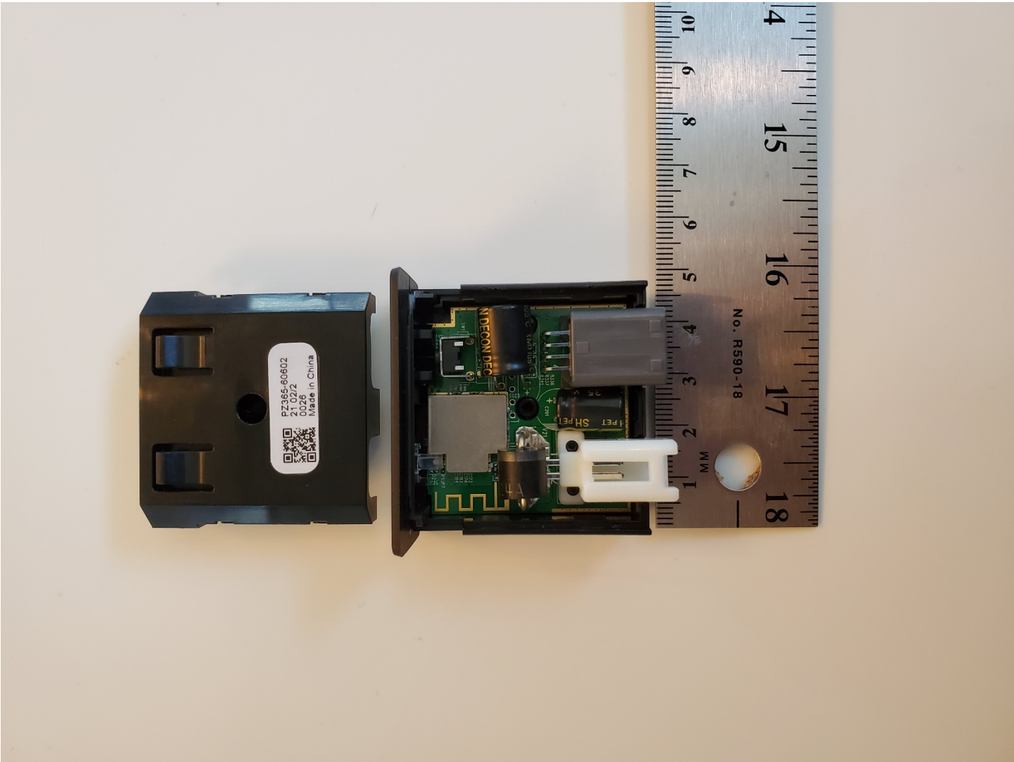
Disassembled View
