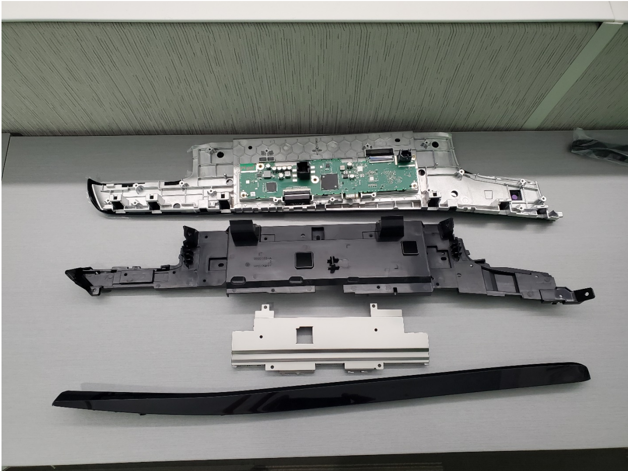
FPDM MY22 WS Disassembled
