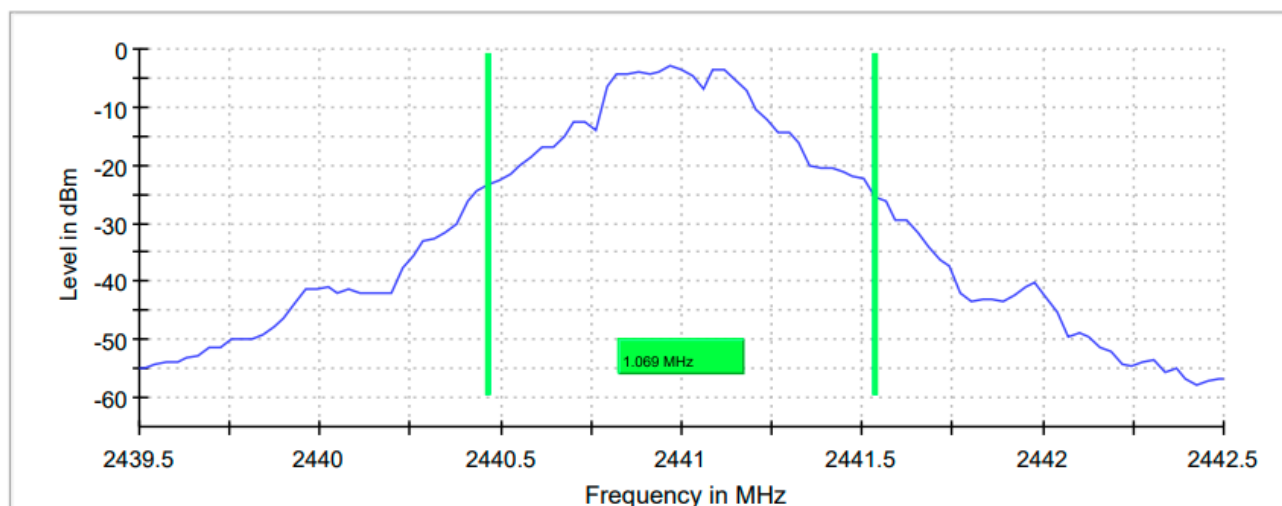
20 dB Bandwidth
