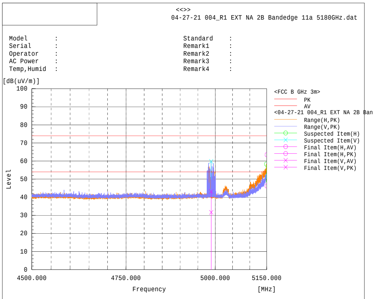
Antenna Polarity & Test Distance: Vertical and Horizontal at 3m
