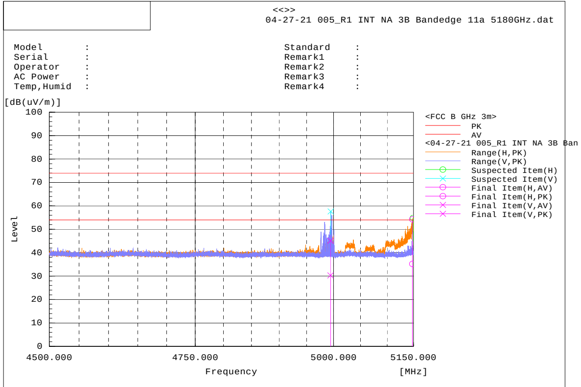
ANTENNA POLARITY & test distance: HORIZONTAL& Vertical at 3 m
