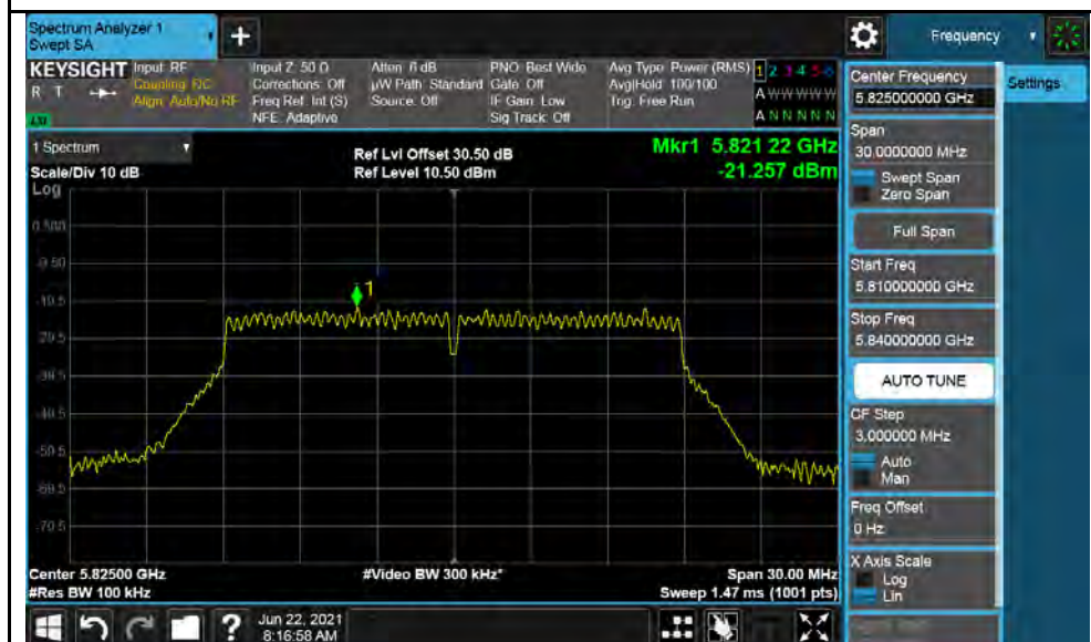
802.11n-HT20-5825MHz
