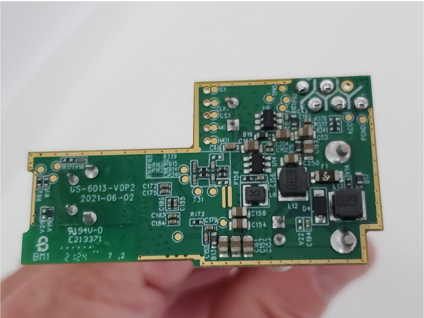
PCBA Bottom View
