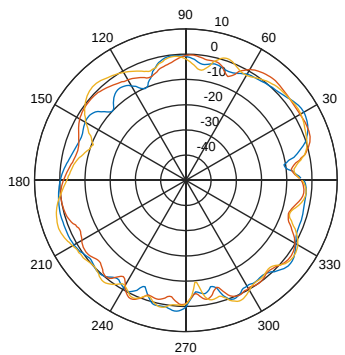
Elevation angle::220 Grad, "Horizontal+Vertical Polarisation"
