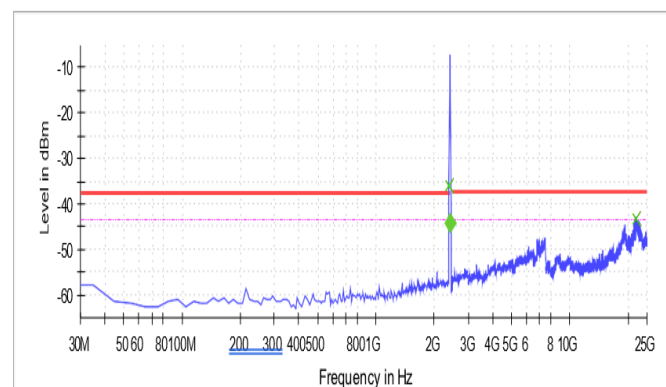
Spurious
