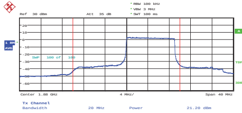
20 MHz – Ch: 18900 – RB# 50 RB Pos: 99
