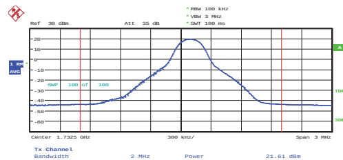
1.4 MHz – Ch: 20175– RB# 1 RB Pos: 3
