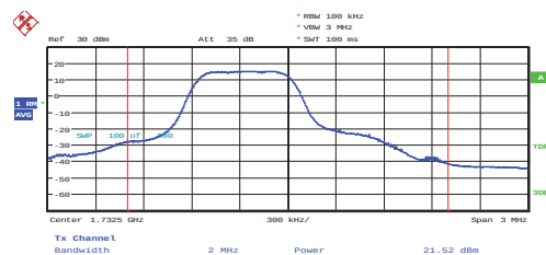
1.4 MHz – Ch: 20175– RB# 3 RB Pos: 0
