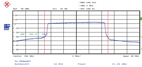
10 MHz – Ch: 23060–RB# 50 RB Pos: 0
