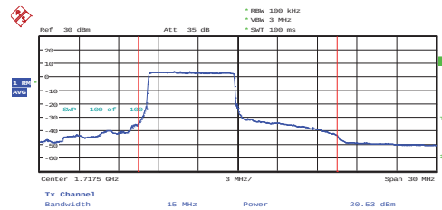
15 MHz – Ch: 20025–RB# 36 RB Pos: 0
