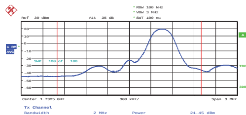
1.4 MHz – Ch: 20175– RB# 1 RB Pos: 5
