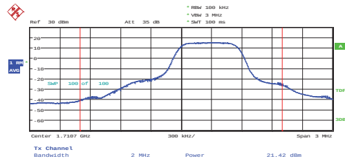
1.4 MHz – Ch: 19957 – RB# RB Pos: 3
