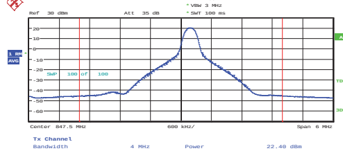
3 MHz – Ch: 20635 – RB# 1 RB Pos: 8
