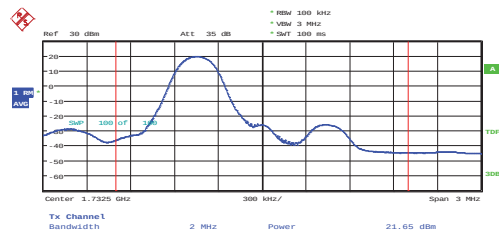
1.4 MHz – Ch: 20175– RB# 1 RB Pos: 0
