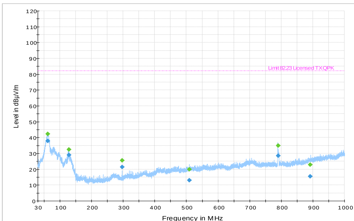
Figure 1: Radiated Spurious Emission 30MHz-1GHz –LTE Band 14-QPSK- 5MHz-Low CH- 790.5MHz
