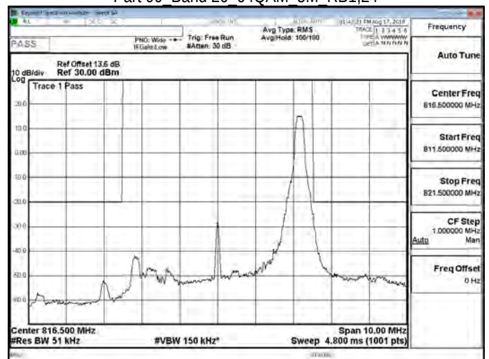
Part 90 Band 26 64QAM 5M RB1,24
