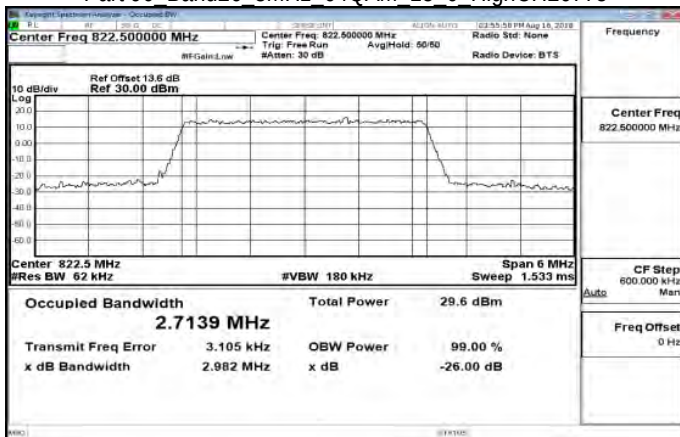
Part 90 Band26 3MHz 64QAM 15 0 HighCH26775
