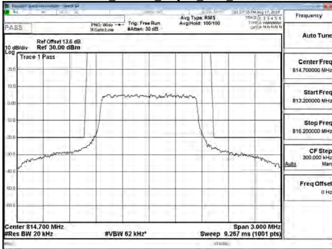
Part 90 Band 26 64QAM 1.4M RB1,0
