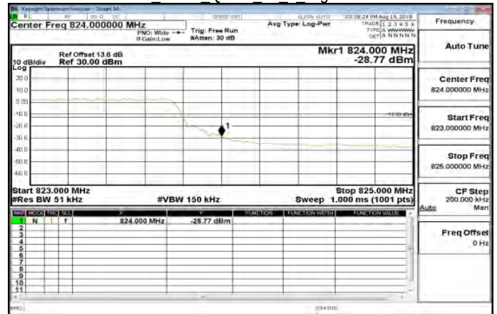
Band26 10MHz QPSK 1 0 LowCH26740
