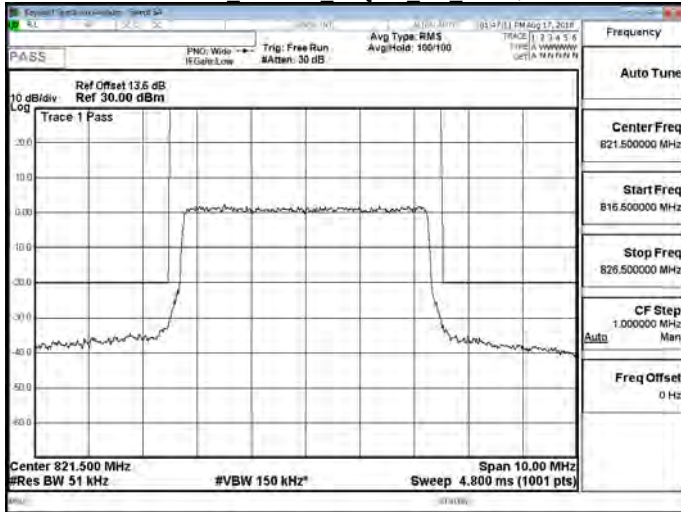
Part 90 Band 26 QPSK 10M RB1,0
