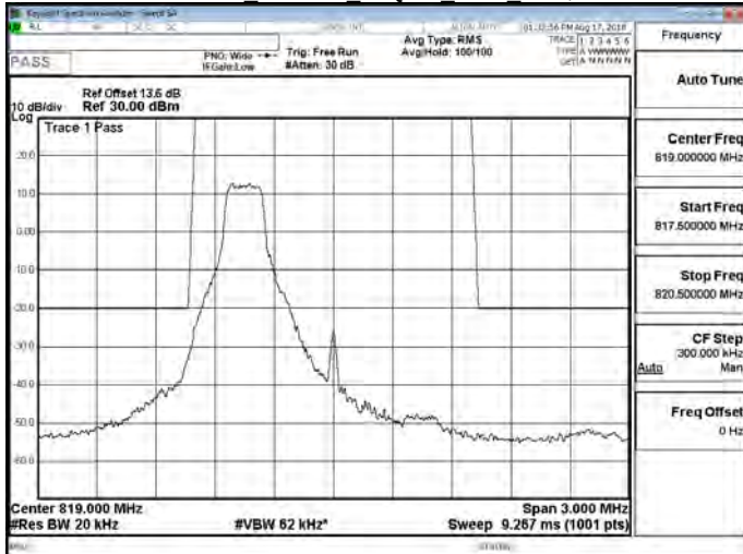
Part 90 Band 26 64QAM 1.4M RB1,5
