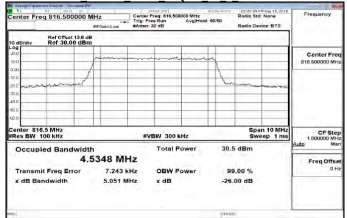
Part 90 Band26 5MHz 64QAM 25 0 MidCH26740
