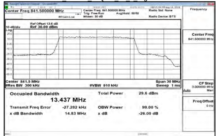
Band26 15MHz 16QAM 75 0 HighCH26965
