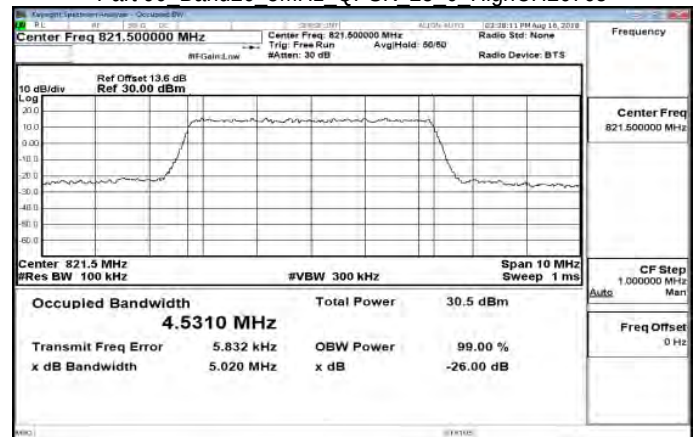
Part 90 Band26 5MHz QPSK 25 0 HighCH26765
