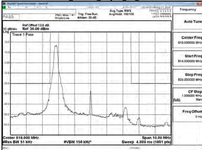
Part 90 Band 26 64QAM 5M RB1,24
