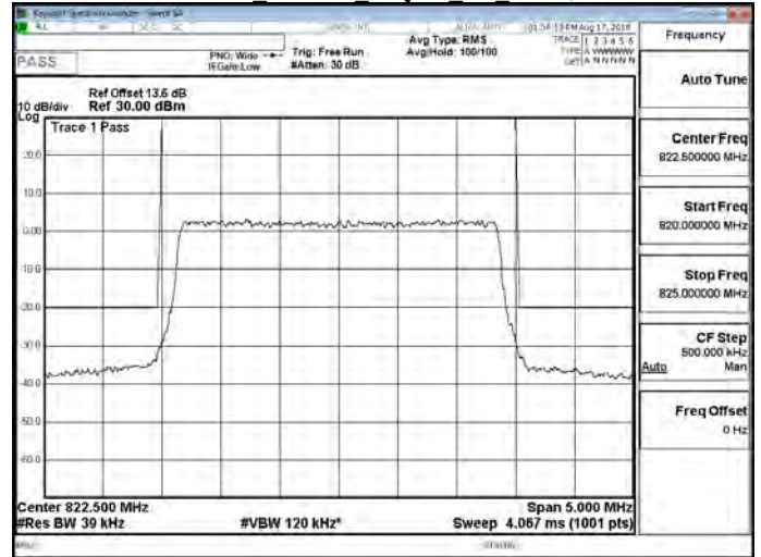
Part 90 Band 26 QPSK 5M RB1,0
