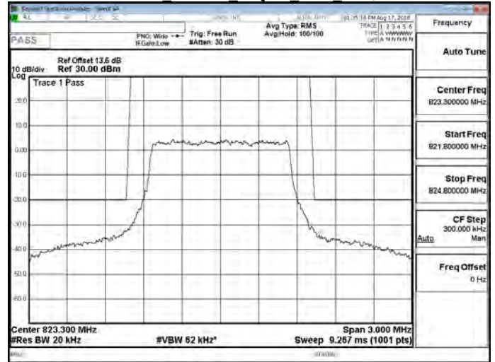
Part 90 Band 26 64QAM 1.4M RB1,0
