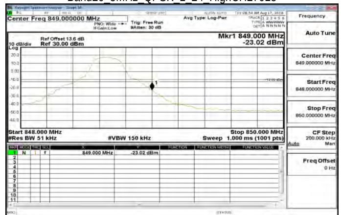
Band26 5MHz QPSK 1 24 HighCH27015
