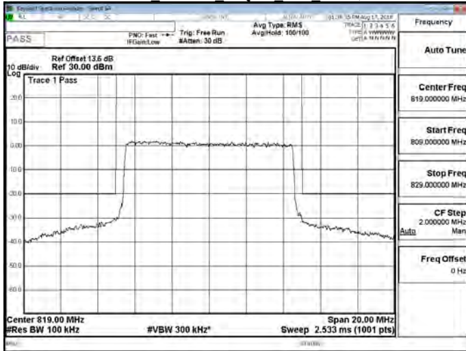
Part 90 Band 26 64QAM 10M RB1,0
