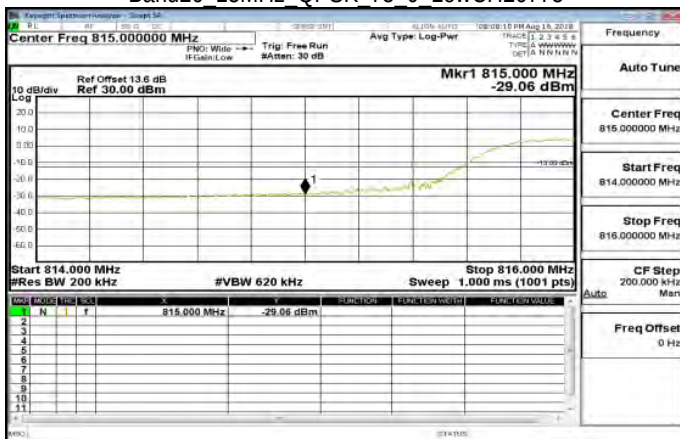
Band26 15MHz QPSK 75 0 LowCH26775
