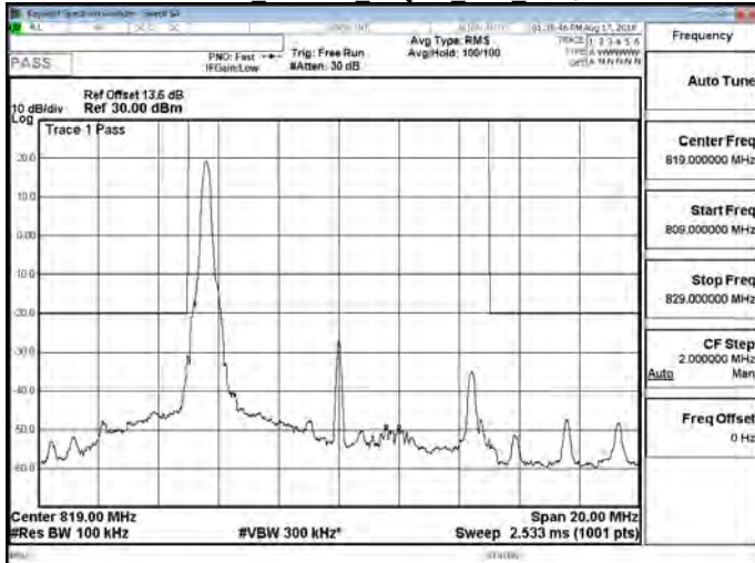
Part 90 Band 26 64QAM 10M RB1,49
