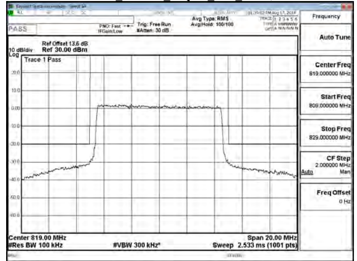
Part 90 Band 26 64QAM 10M RB50,0
