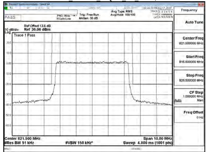
Part 90 Band 26 64QAM 5M RB1,0
