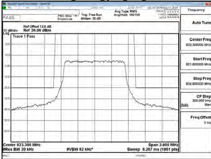
Part 90 Band 26 16QAM 1.4M RB1,0
