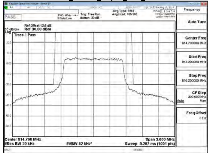
Part 90 Band 26 16QAM 1.4M RB1,0
