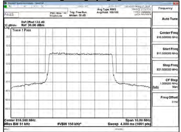
Part 90 Band 26 16QAM 5M RB1,0
