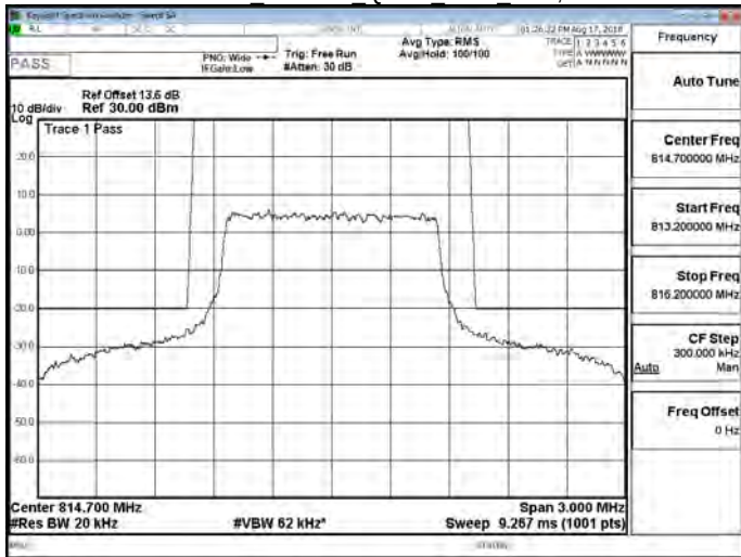
Part 90 Band 26 QPSK 1.4M RB1,0
