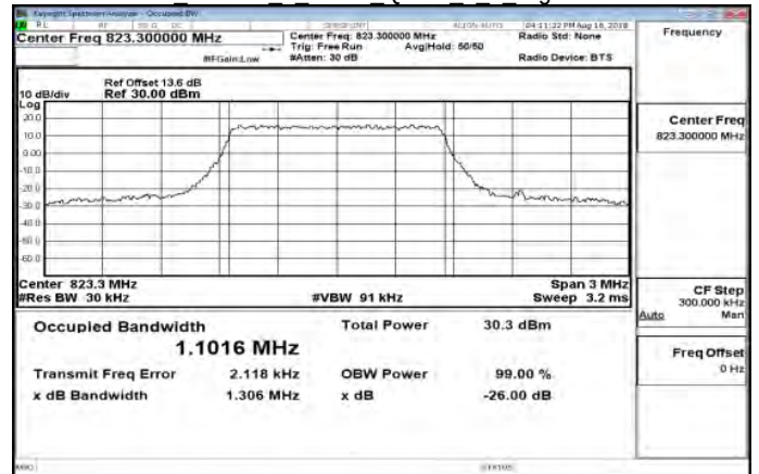
Part 90 Band26 1 4MHz QPSK 6.0 HighCH26783
