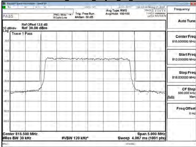
Part 90 Band 26 16QAM 3M RB1,0
