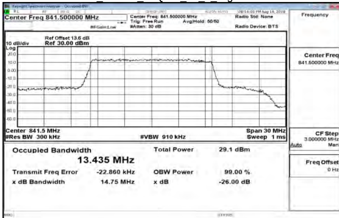
Band26 15MHz 64QAM 75.0 HighCH26965
