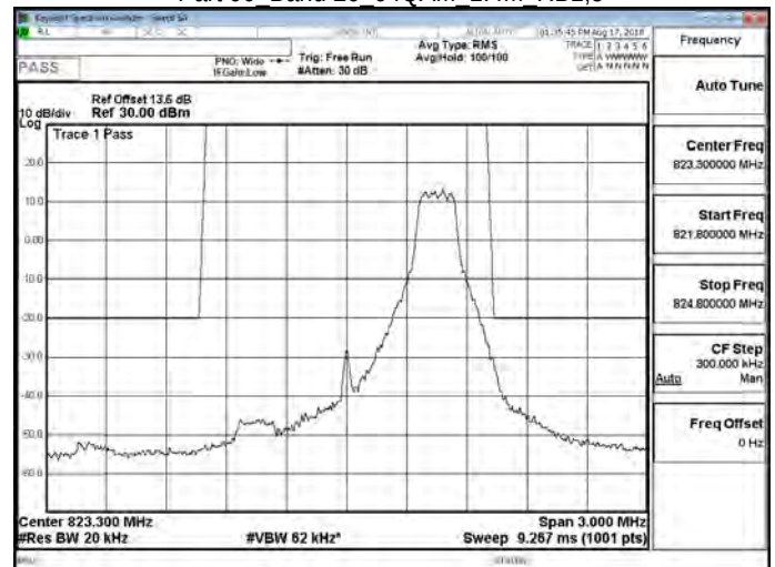
Part 90 Band 26 64QAM 1.4M RB1,5
