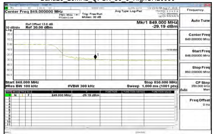
Band26 10MHz QPSK 50 0 HighCH26990
