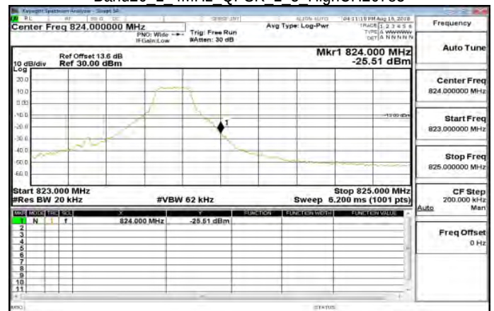
Band26 1 4MHz QPSK 1 5 HighCH26783
