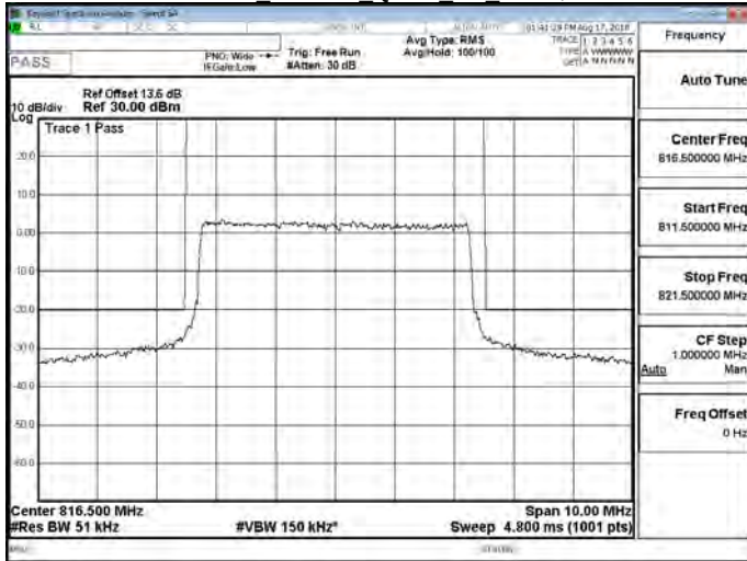
Part 90 Band 26 QPSK 5M RB1,0
