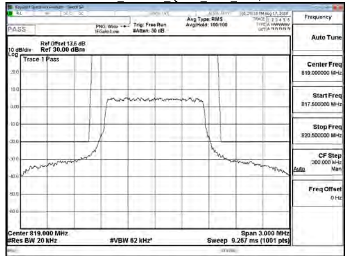
Part 90 Band 26 QPSK 1.4M RB1,0
