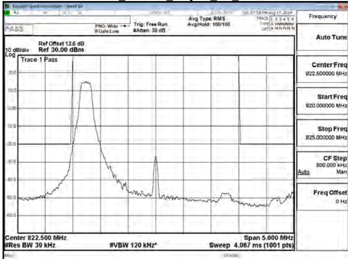
Part 90 Band 26 64QAM 3M RB1,14
