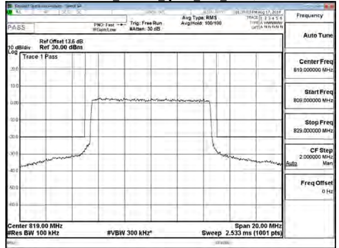
Part 90 Band 26 16QAM 10M RB1,0
