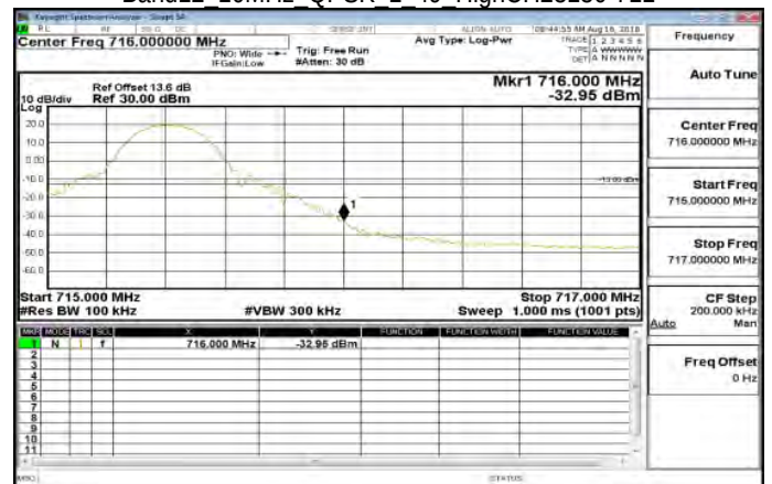
Band12 10MHz QPSK 1 49 HighCH23130-711
