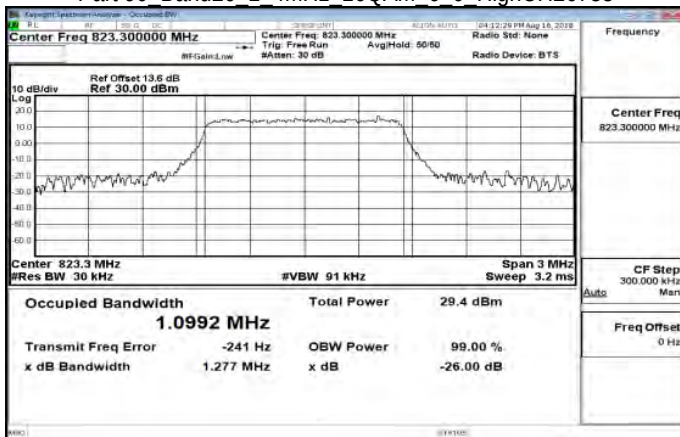
Part 90 Band26 1 4MHz 16QAM 6 0 HighCH26783
