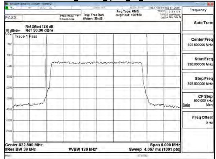
Part 90 Band 26 16QAM 3M RB1,0
