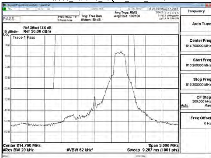
Part 90 Band 26 16QAM 1.4M RB1,5
