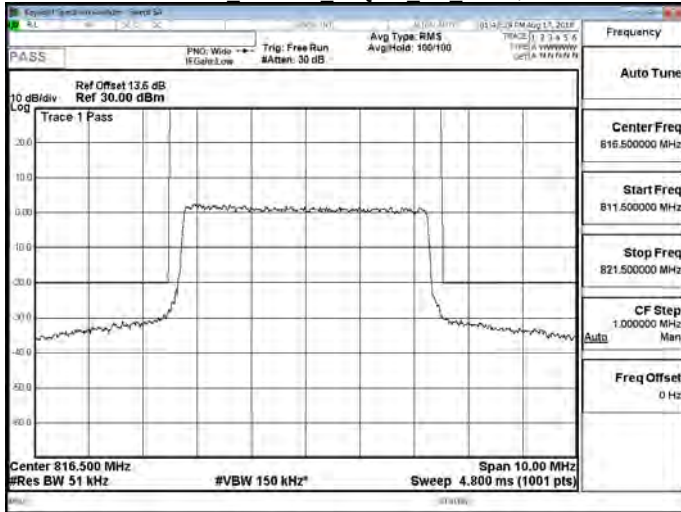
Part 90 Band 26 64QAM 5M RB1,0
