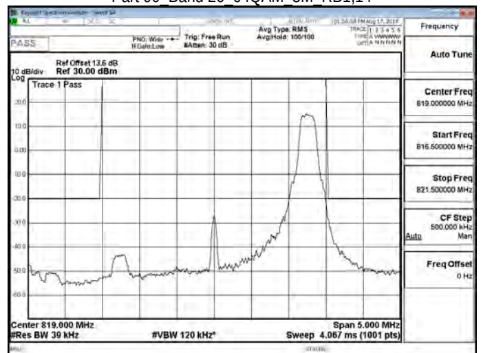
Part 90 Band 26 64QAM 3M RB1,14
