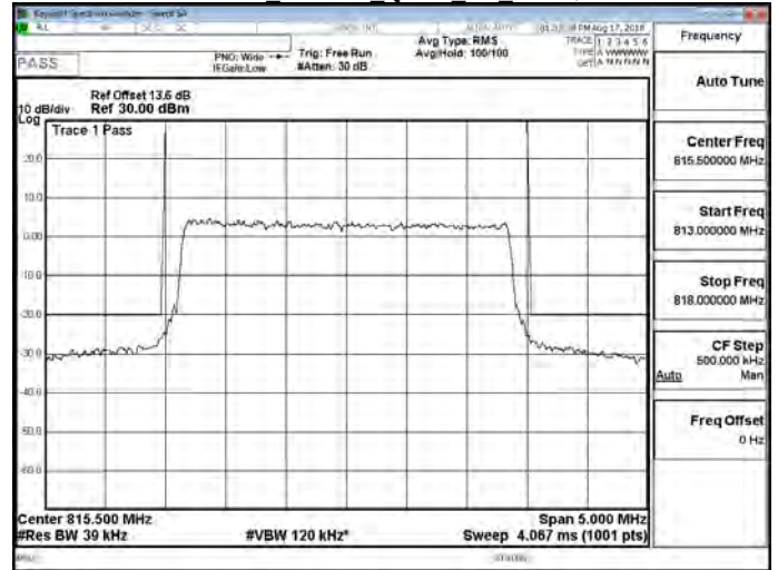
Part 90 Band 26 QPSK 3M RB1,0
