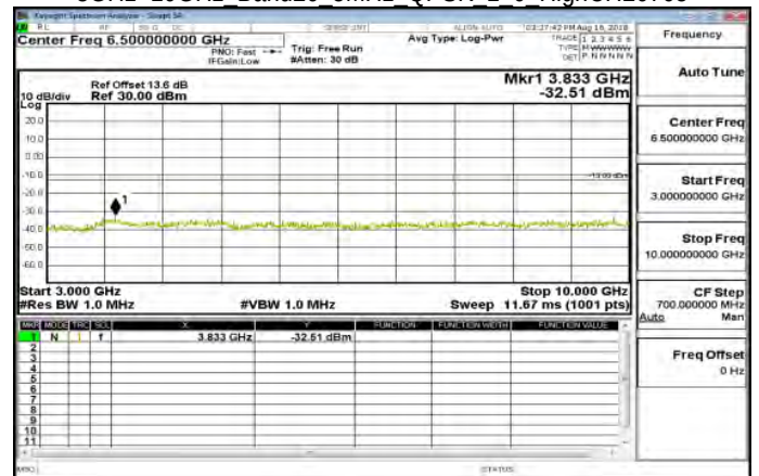
3GHz~10GHz Band26 5MHz QPSK 1 0 HighCH26765
