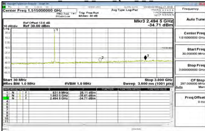
30MHz~3GHz Band26 1 4MHz QPSK 1 0 MidCH26865
