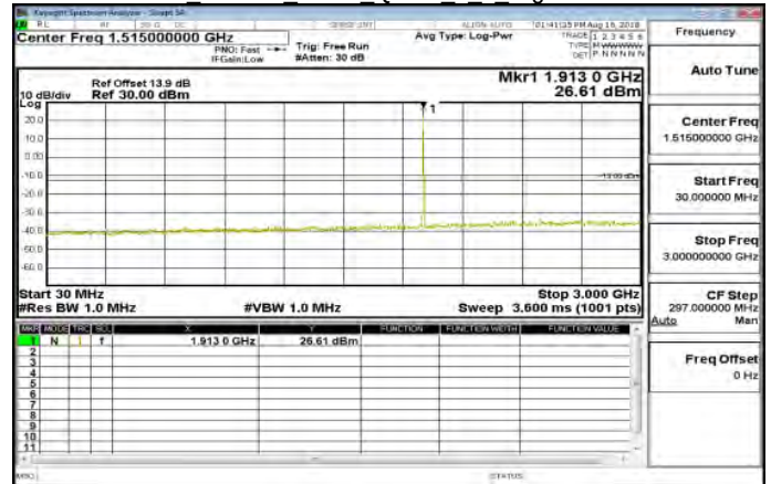
30MHz~3GHz Band25 3MHz QPSK 1 0 HighCH26675-1913.5
