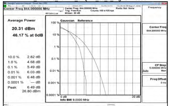
LTE Band26 10MHz 64QAM 50 0 HighCH26990
