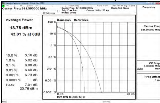
LTE Band26 15MHz 64QAM 75 0 HighCH26965
