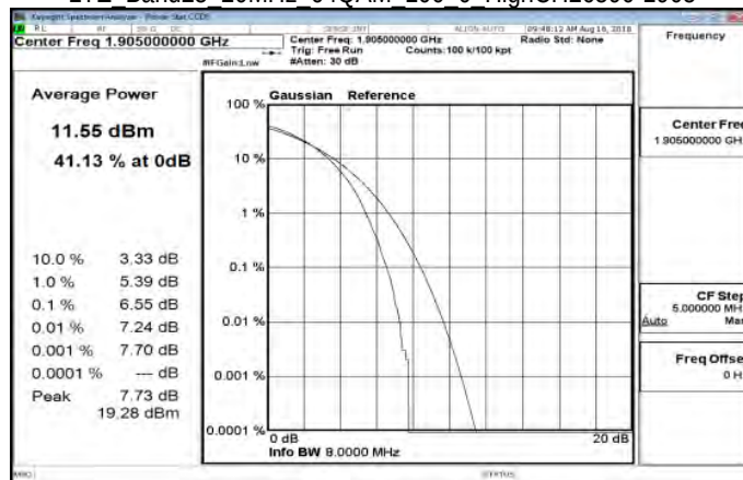
LTE Band25 20MHz 64QAM 100 0 HighCH26590-1905
