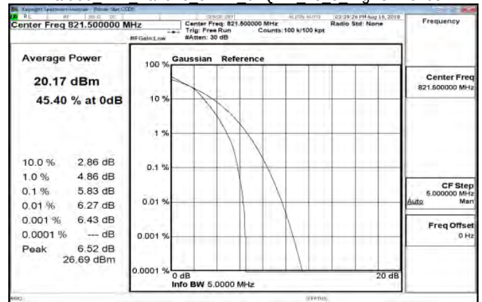
Part 90 LTE Band26 5MHz 64QAM 25 0 HighCH26765
