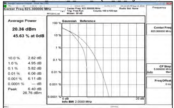
Part 90 LTE Band26 1 4MHz 64QAM 6 0 HighCH26783
