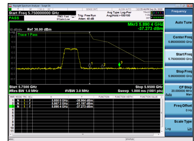
U-NII-3 ,Plot 1,Band Edge-802.11n(20 Hz),5825MHz,Ant1
