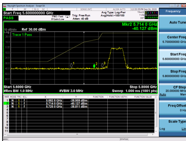
U-NII-3 ,Plot 1,Band Edge-802.11n(20 Hz),5745MHz,Ant1
