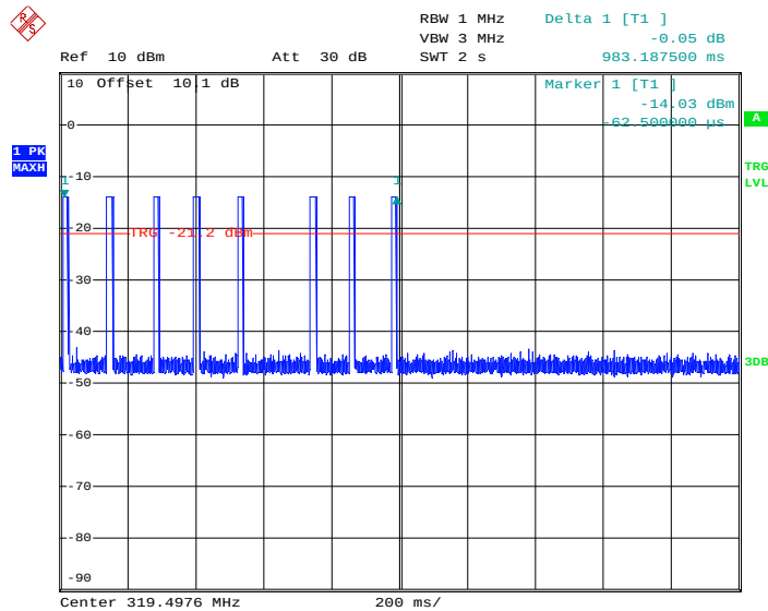
Figure 7.4.2-2: Duration of Transmission – 200 ms
