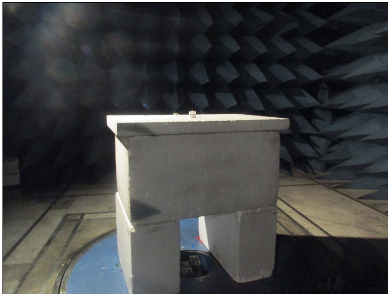
Figure 5: Radiated Emissions above 1 GHz – Front View – EUT Upright
