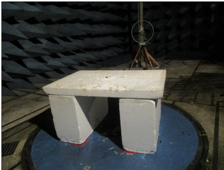
Figure 2: Radiated Emissions 9 kHz to 30 MHz – Back View – EUT Upright
