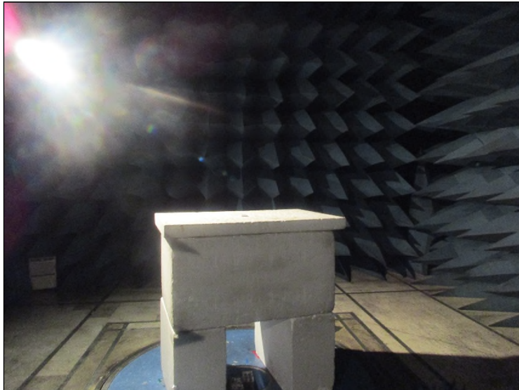
Figure 11: Radiated Emissions above 1 GHz – Front View – EUT Flat
