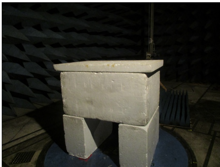
Figure 12: Radiated Emissions above 1 GHz – Back View – EUT Flat
