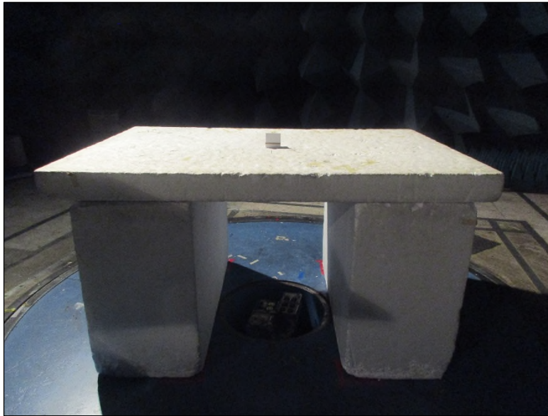
Figure 1: Radiated Emissions below 1 GHz – Front View – EUT Upright
