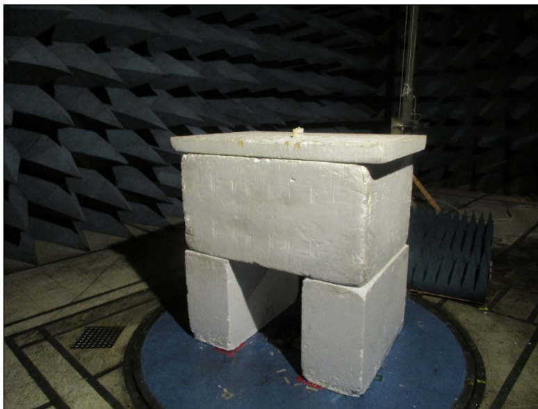
Figure 6: Radiated Emissions above 1 GHz –Back View – EUT Upright
