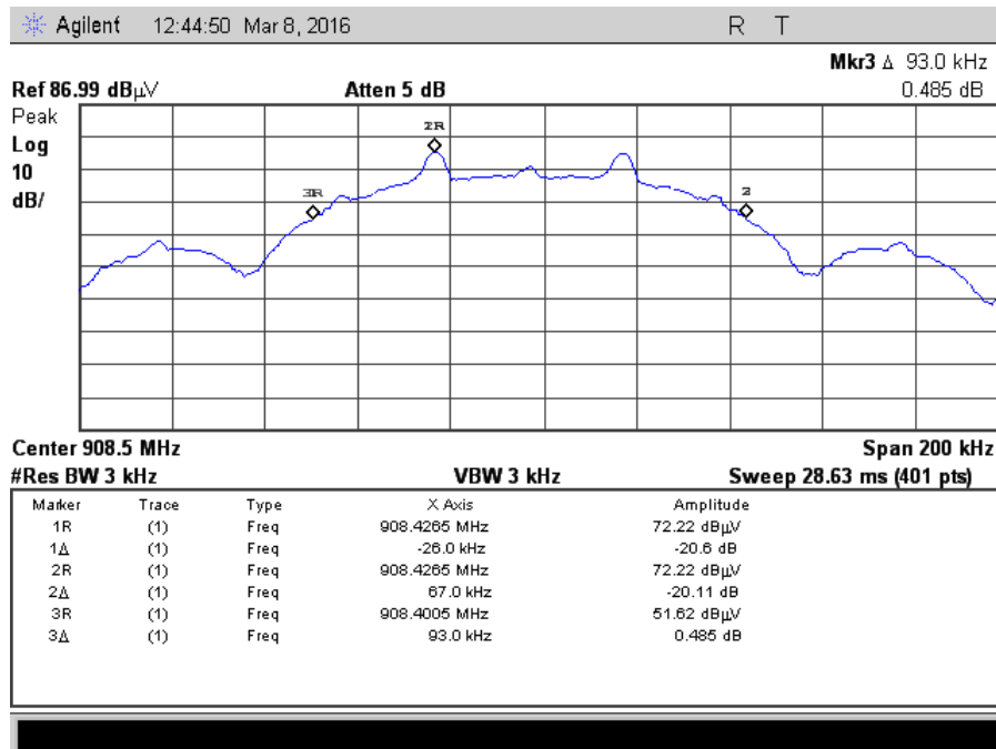
Figure 7.2.2-1: 20dB BW
