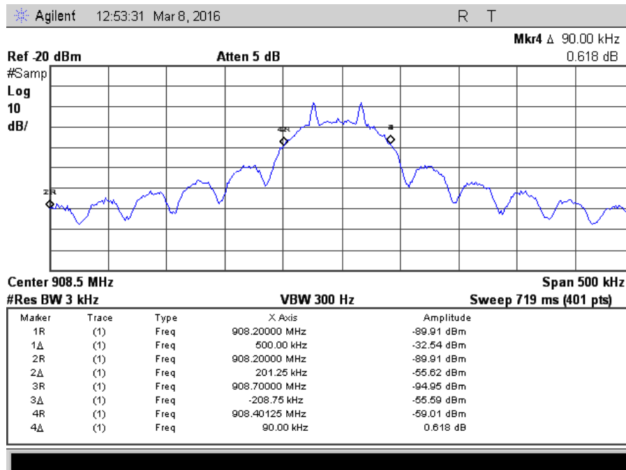
Figure 7.2.2-2: 99% OBW
