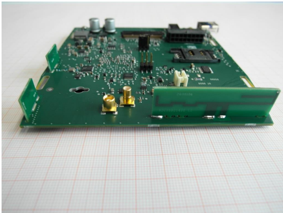
Photo 7 (EUT – Antenna):
