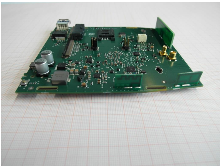
Photo 8 (EUT – Antennas):
