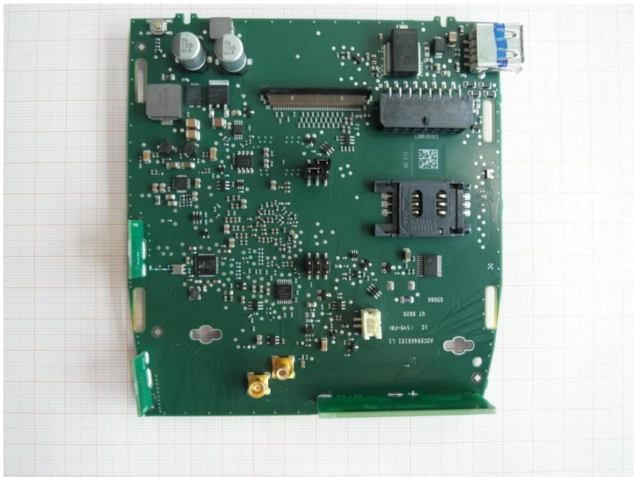
Photo 5 (EUT – rear view of circuitry):
