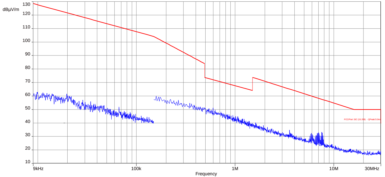
Plot 1: 9 kHz to 30 MHz, GFSK, channel 00, transmit mode
