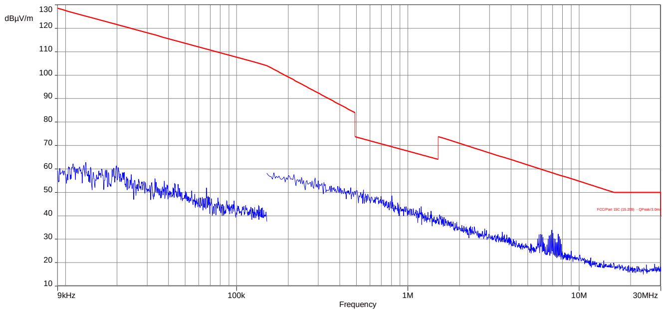
Plot 2: 9 kHz to 30 MHz, GFSK, channel 39, transmit mode
