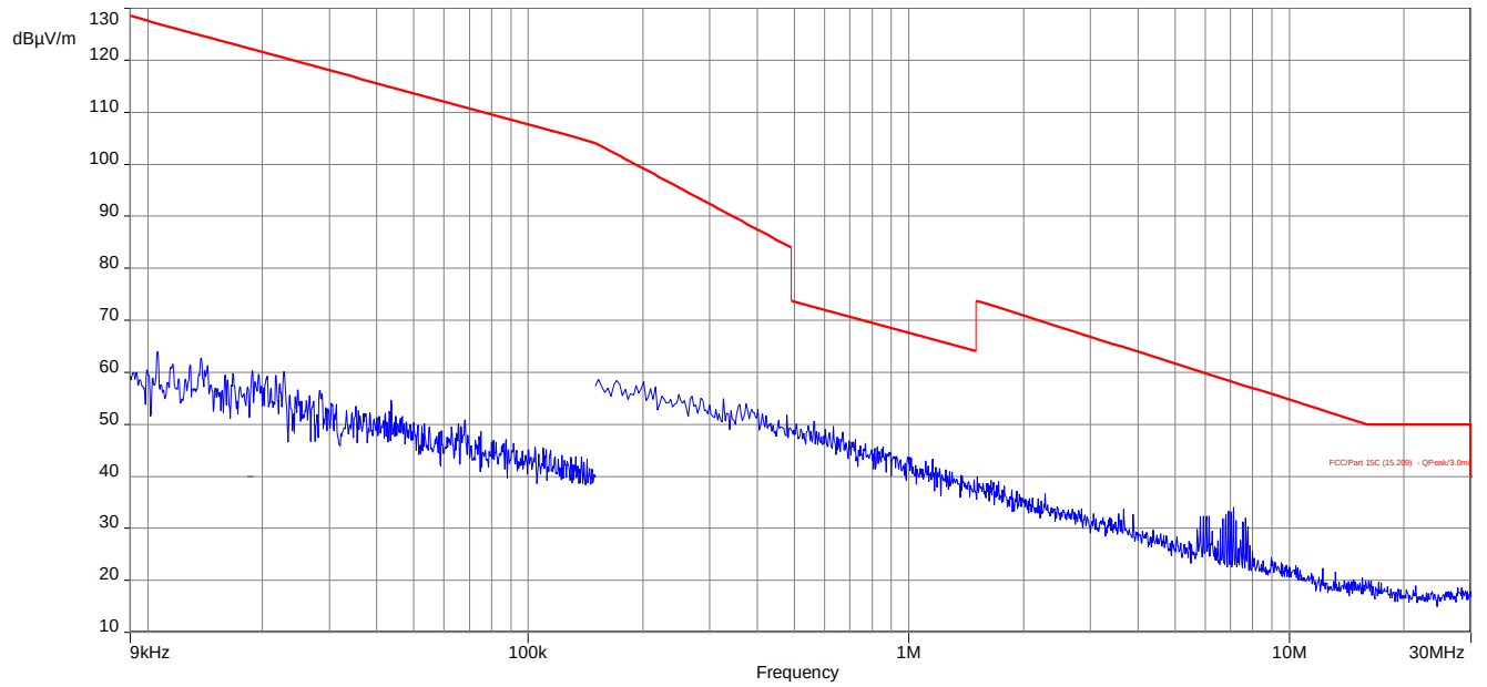
Plot 3: 9 kHz to 30 MHz, GFSK, channel 78, transmit mode
