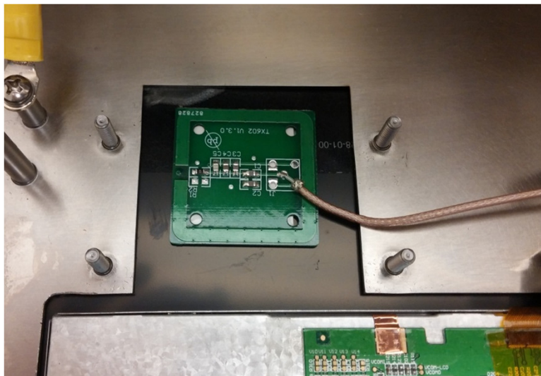
TX602 Antenna installed without shield
