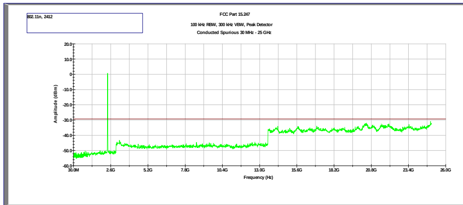
Plot 4.7 Tx @ 2412MHz 802.11n, HT20
