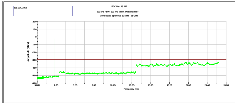
Plot 4.9 Tx @ 2462MHz 802.11n, HT20
