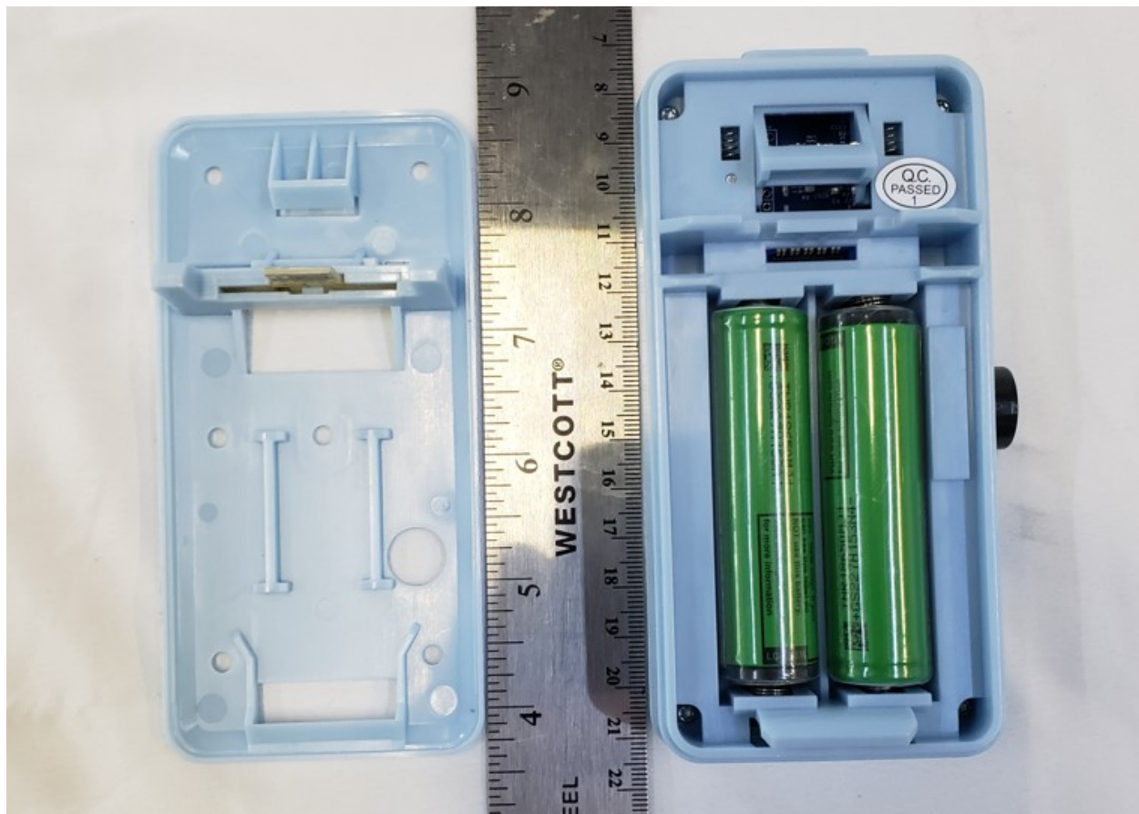
Figure 3. Back of EUT with wall plate removed. (The EUT is marketed with the wall plate removed.)
