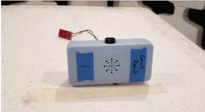
Figure 1. Radiated Emissions Test Setup, Intentional Testing
