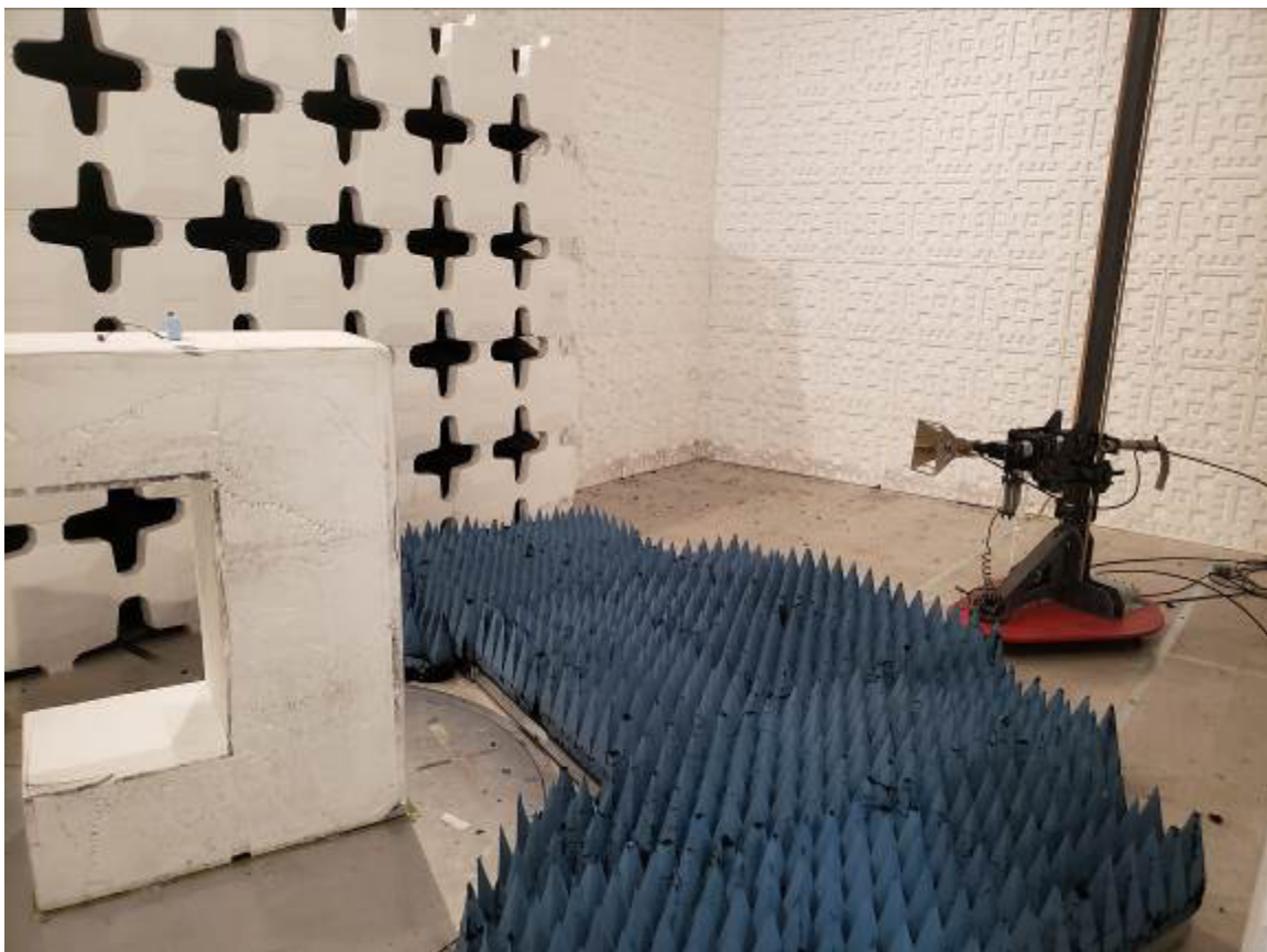
Figure 5. Radiated Emission Test Setup, Intentional, above 1 GHz
