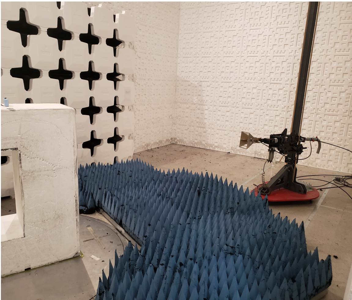
Figure 5. Radiated Emission Test Setup, Intentional, above 1 GHz
