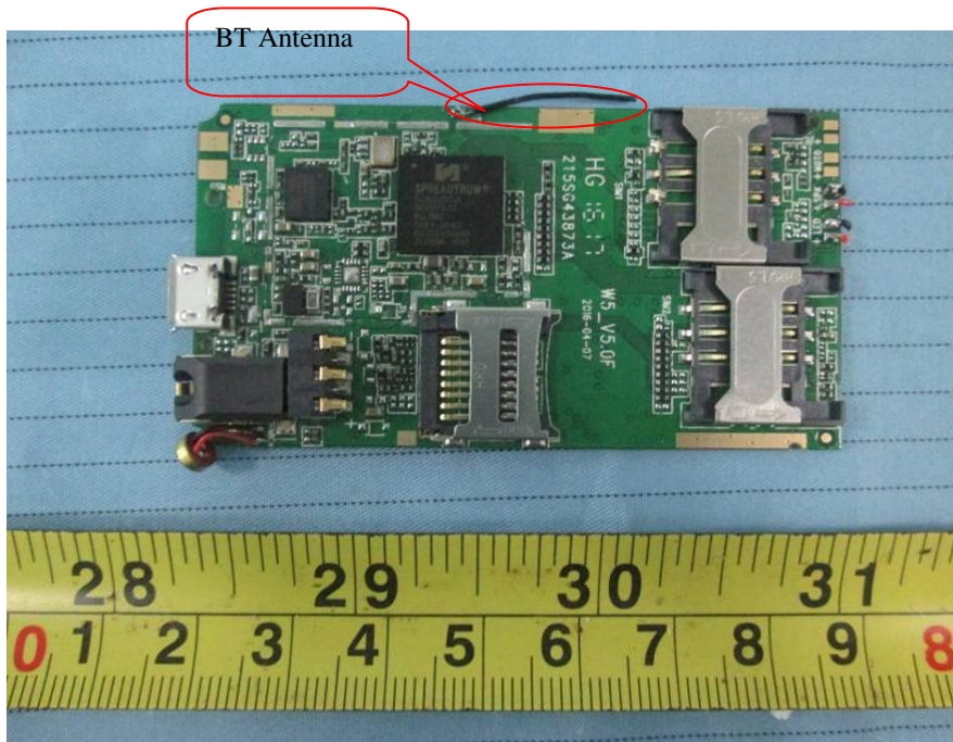
EUT – Main Board Bottom Shielding off View
