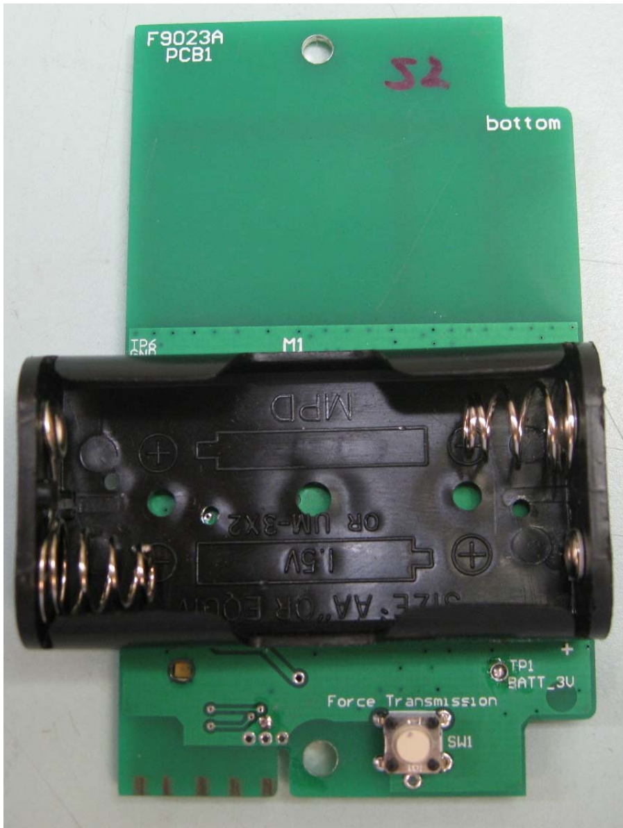
Figure 5: 10850A – PCB Bottom View
