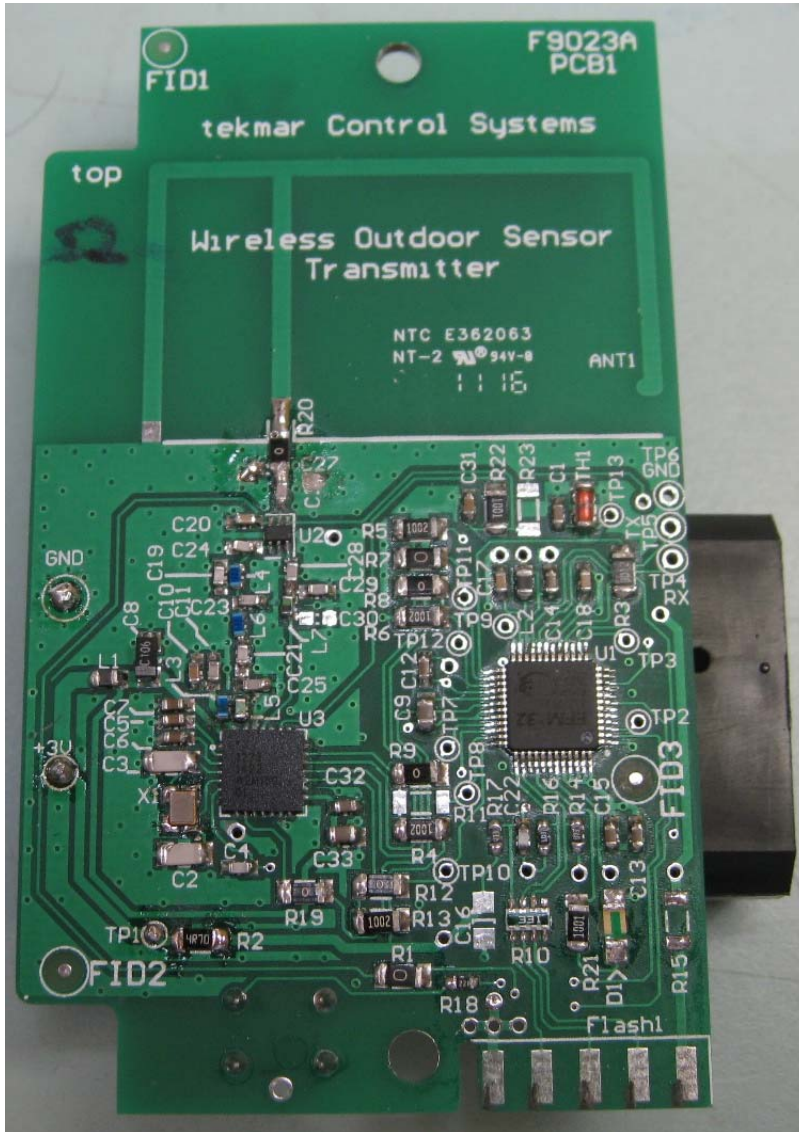
Figure 4: 10850A – PCB Top View
