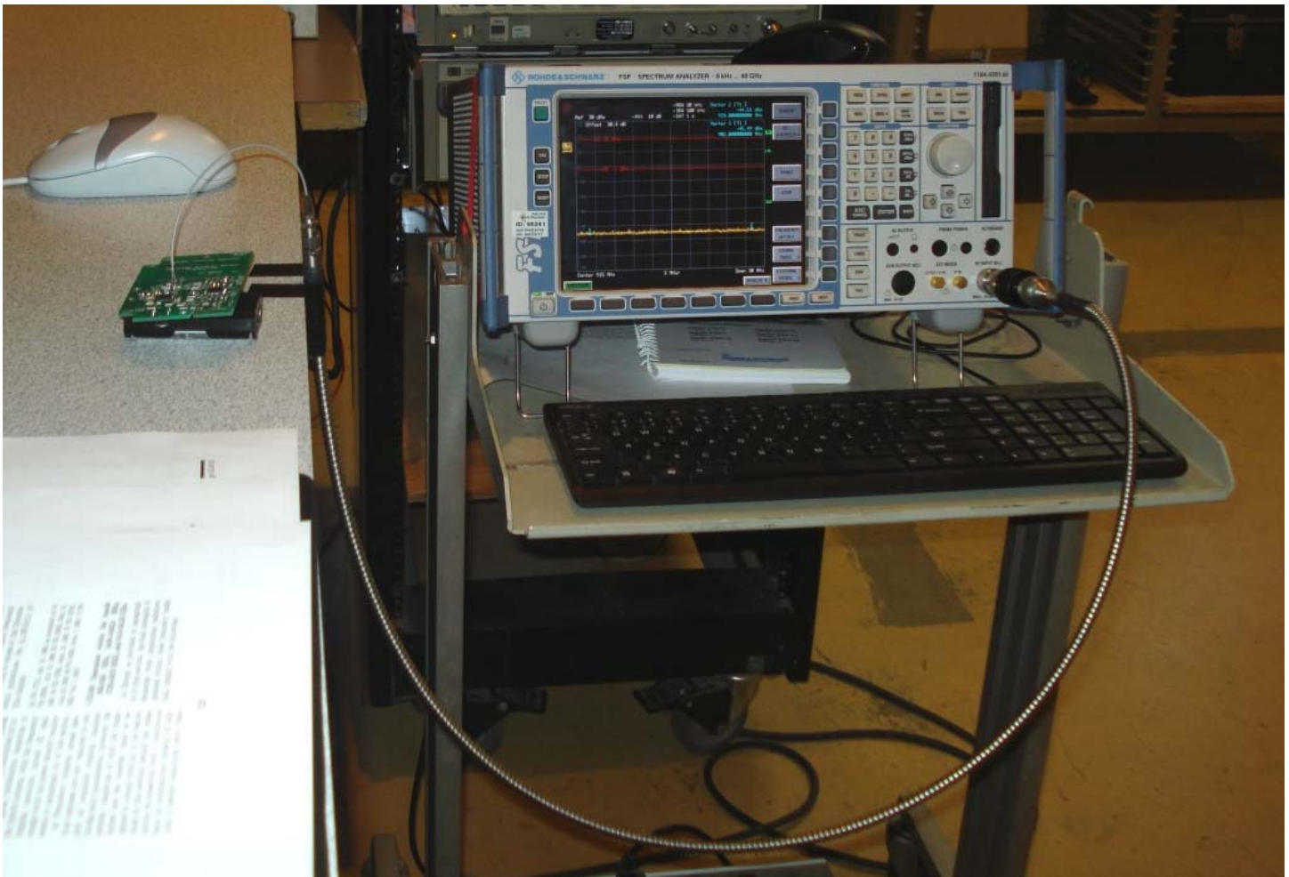
Figure 7: Conducted Measurements
