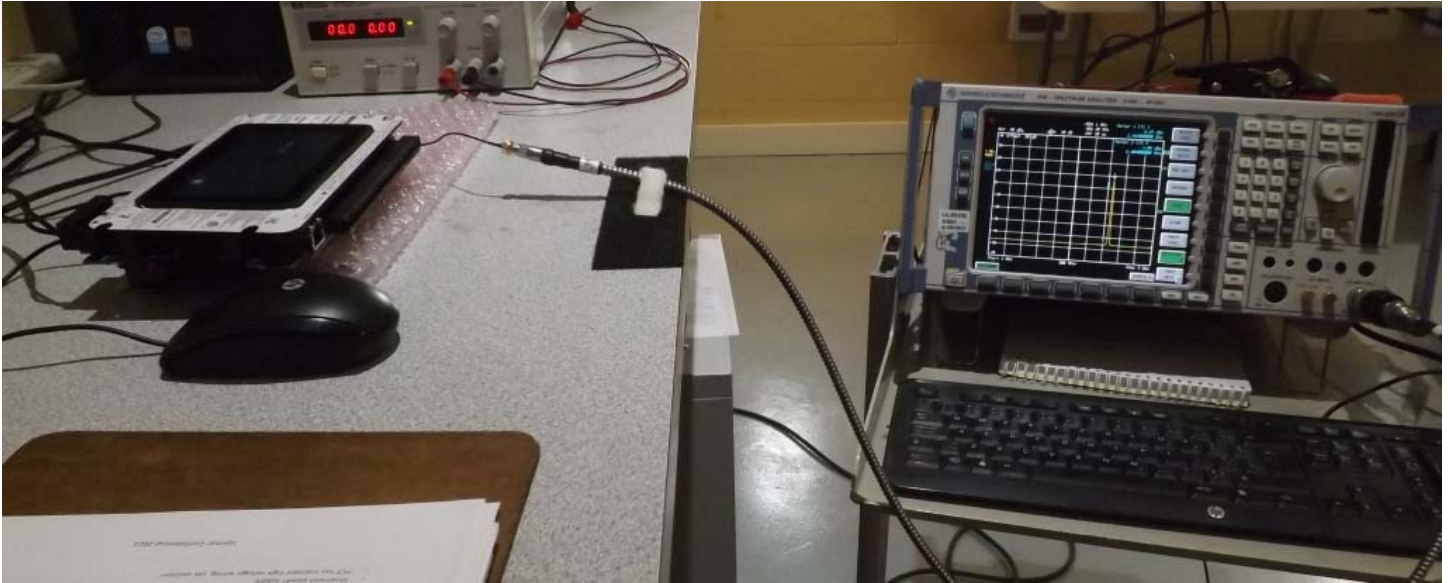
Figure E23.1 – Setup – Conducted Measurements
