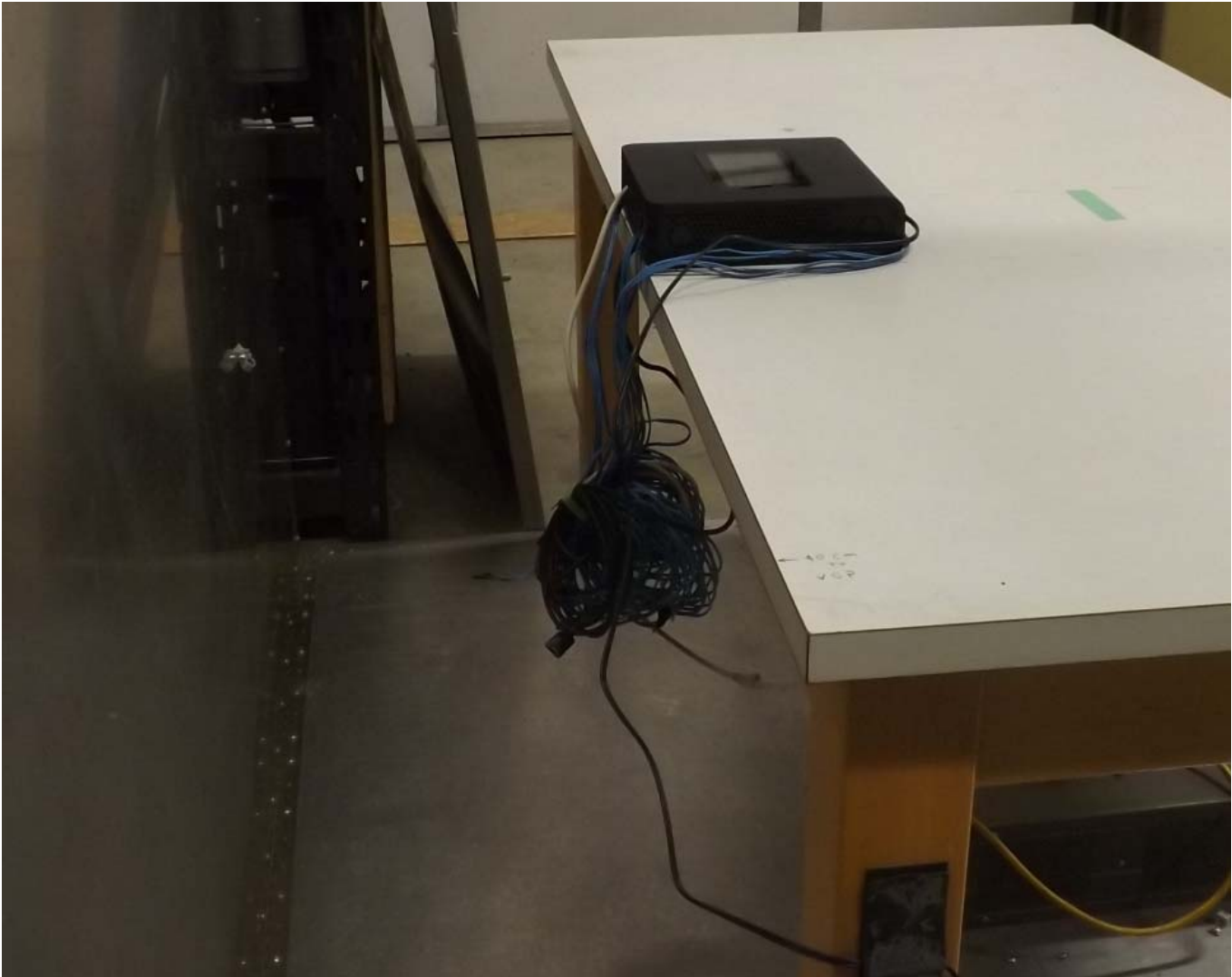
Figure E23.2B – Setup – Line Conducted Emissions
