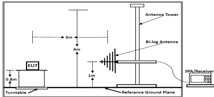
Below 1GHz
