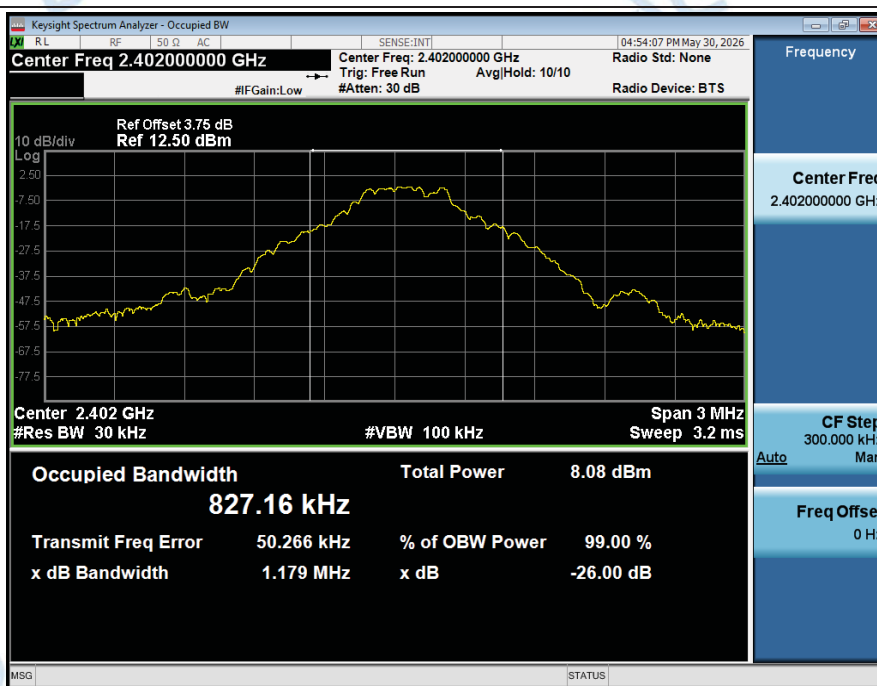
99%_Occupied_Bandwidth_NVNT_ANT1_1-DH5_2402_00
